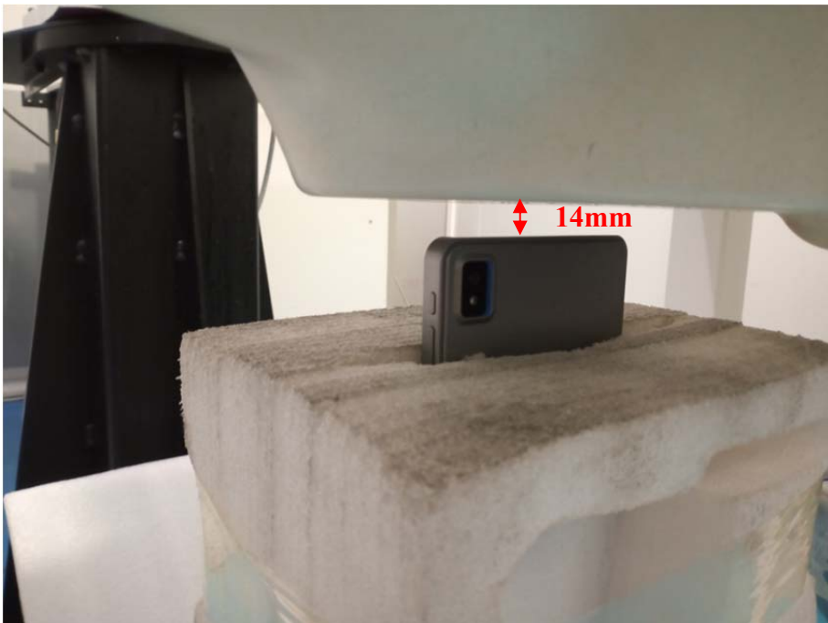
Body Top Setup Photo(14mm)
