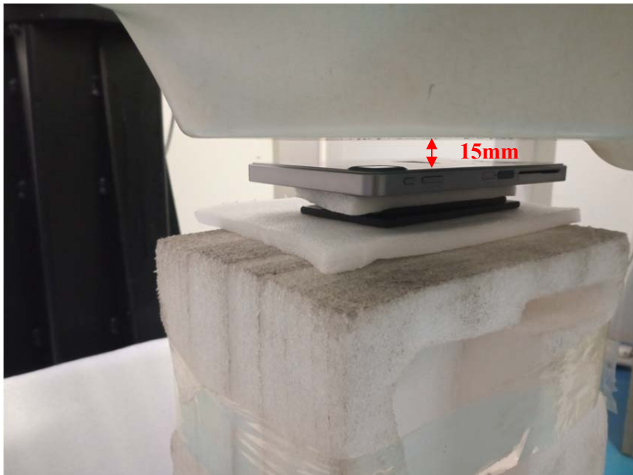
Body Back Setup Photo(15mm)
