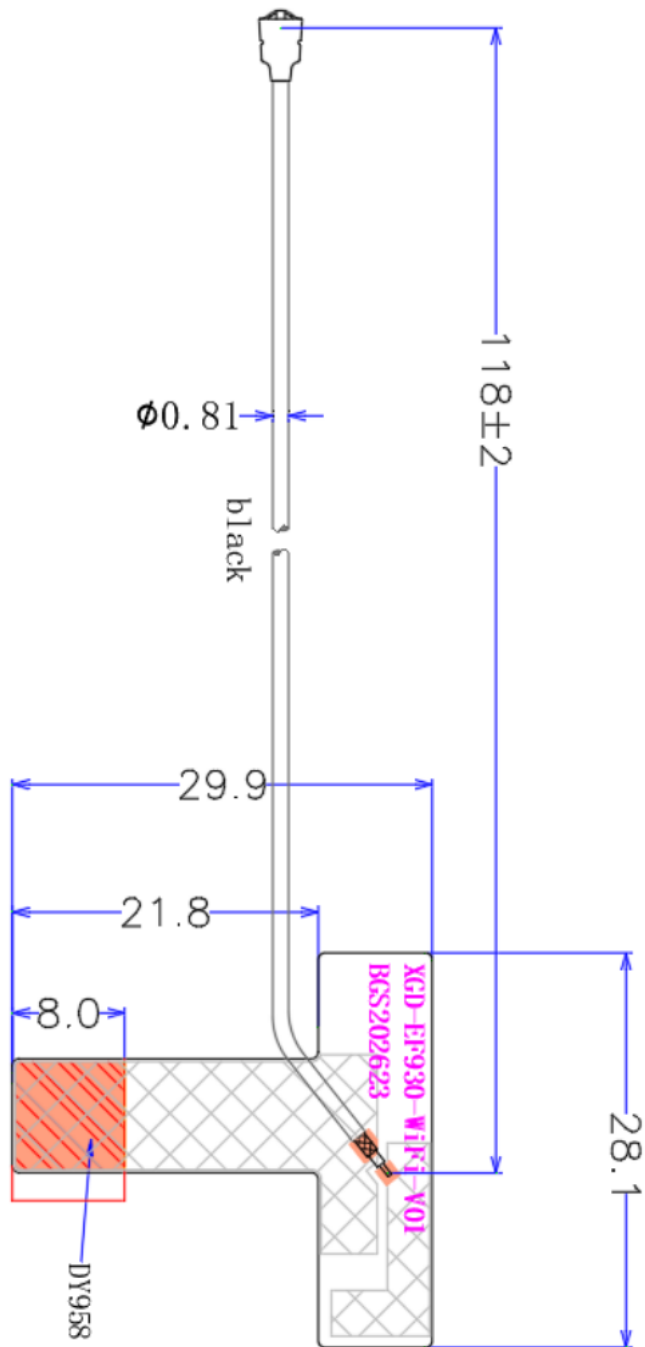
Front view
