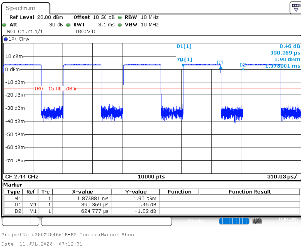
BLE_1M_Middle_Channel
