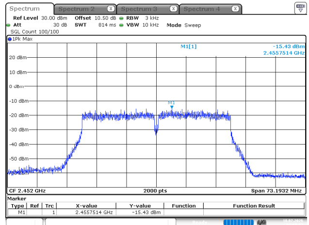
802.11n40_2452MHz
