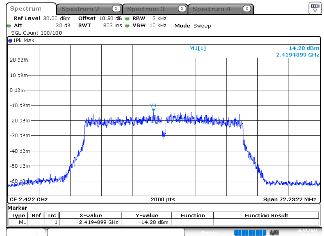
802.11n40_2422MHz
