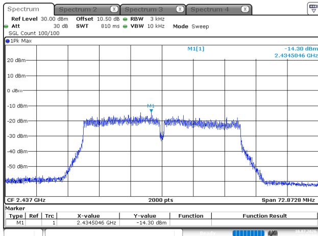
802.11n40_2437MHz
