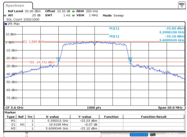
802.11n20_5600MHz
