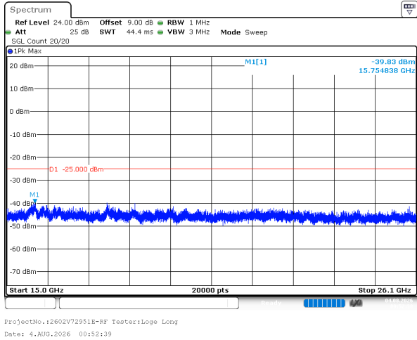
20MHz_High_QPSK_1@0(15GHz~26.1GHz)
