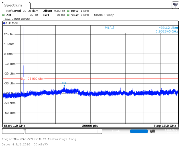
10MHz_High_QPSK_1@0(1GHz~15GHz)
