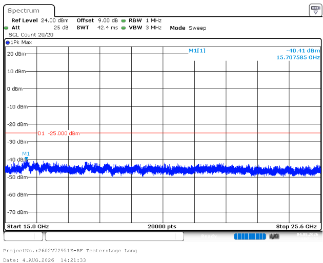
20MHz_High_QPSK_1@0(15GHz~25.6GHz)
