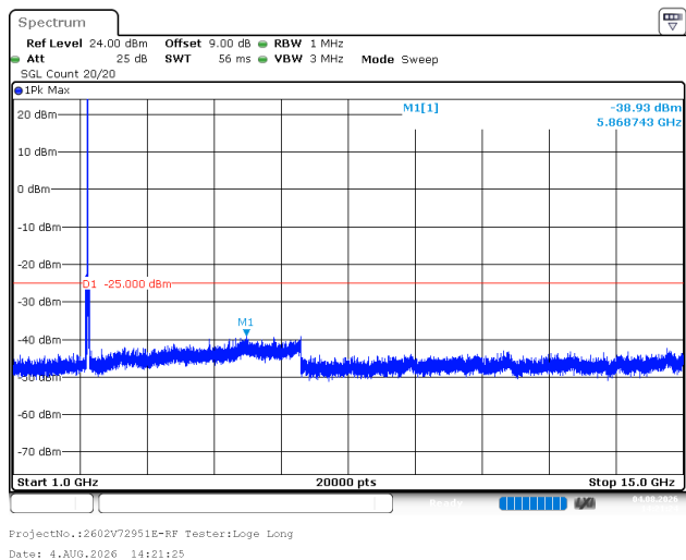
20MHz_High_QPSK_1@0(1GHz~15GHz)
