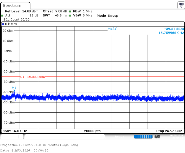
15MHz_Middle_QPSK_1@0(15GHz~25.95GHz)
