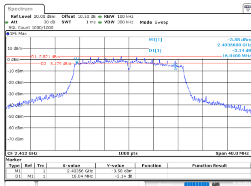
n20_2412MHz_Chain 0
