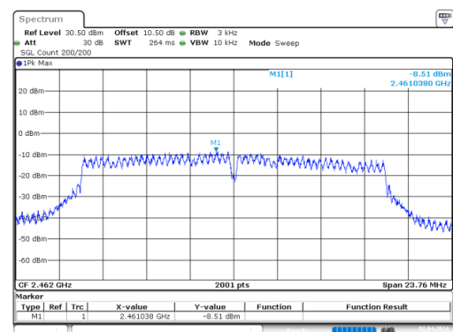
g_2462MHz_Chain 0
