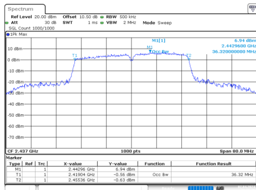
N40_2437MHz_Chain 0
