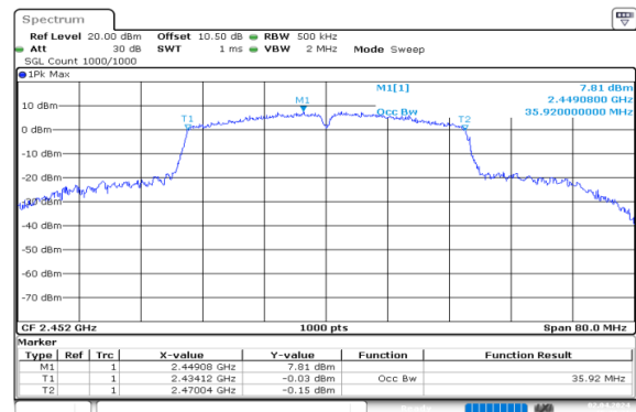
N40_2452MHz_Chain 0
