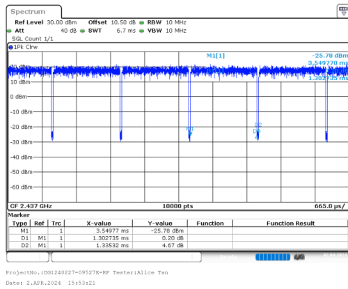
n20_2437MHz_Chain 0
