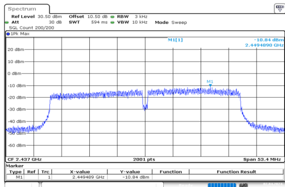
N40_2437MHz_Chain 0
