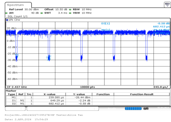
N40_2437MHz_Chain 0
