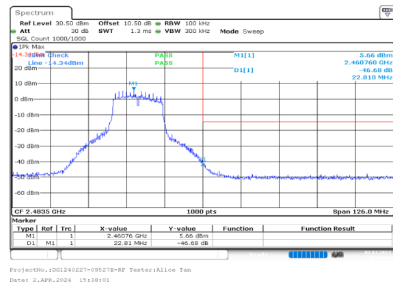
g_2462MHz_Chain 0
