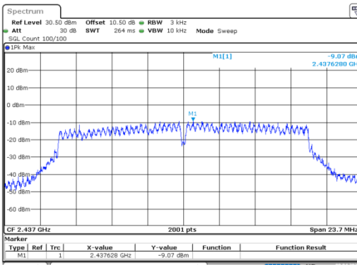
g_2437MHz_Chain 0
