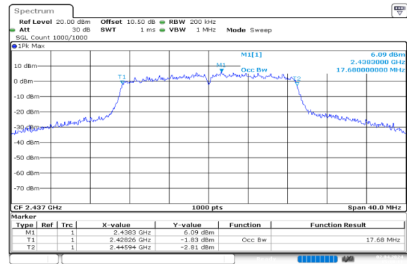
n20_2437MHz_Chain 0
