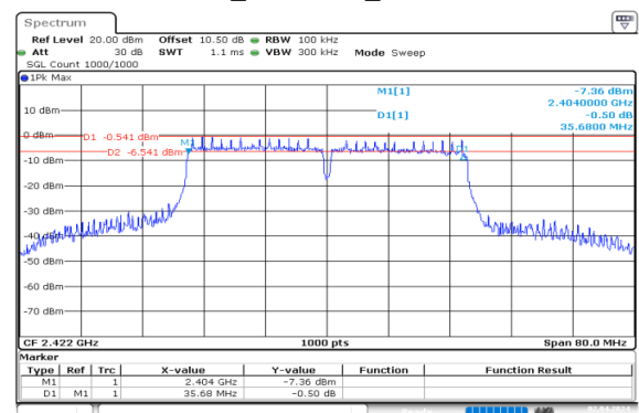
N40_2422MHz_Chain 0
