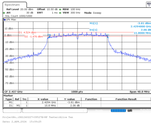
g_2437MHz_Chain 0
