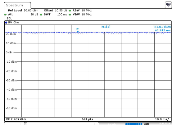
g_2437MHz_Chain 0
