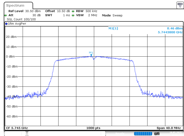
802.11n20_5745MHz
