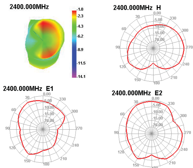
at 2400MHz
