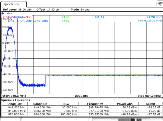
EDGE_High_8PSK
