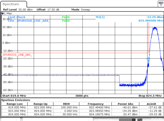
EDGE_Low_8PSK
