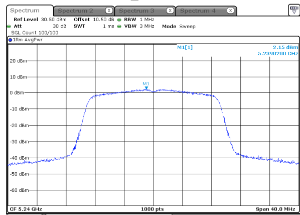
n20_5240MHz
