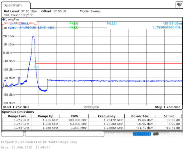
3MHz_High_16QAM_1@14
