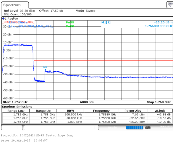
3MHz_High_16QAM_15@0
