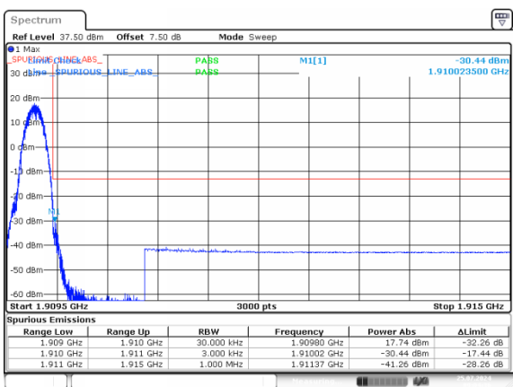
EDGE_High_Solt1 -30.44dBm
