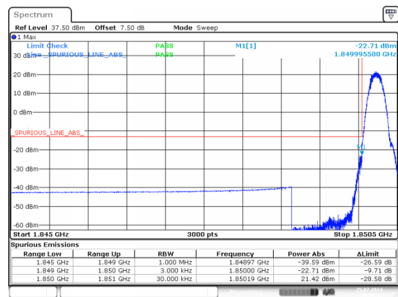
GPRS_Low_Solt1 -22.71dBm
