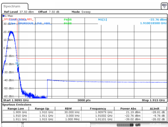
GPRS_High_Solt1 -22.76dBm
