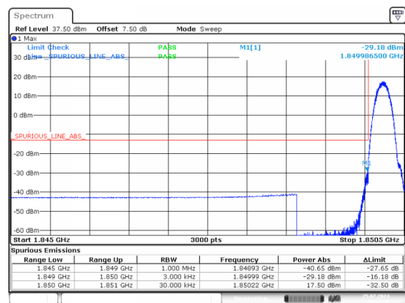
EDGE_Low_Solt1 -29.18dBm
