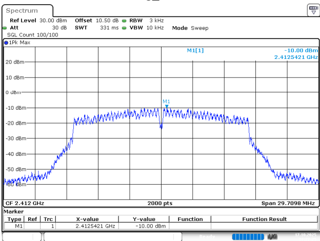
802.11g_2412MHz
