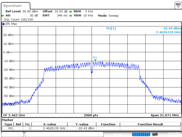
802.11g_2462MHz
