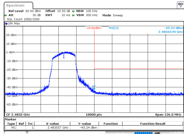
802.11g_2462MHz
