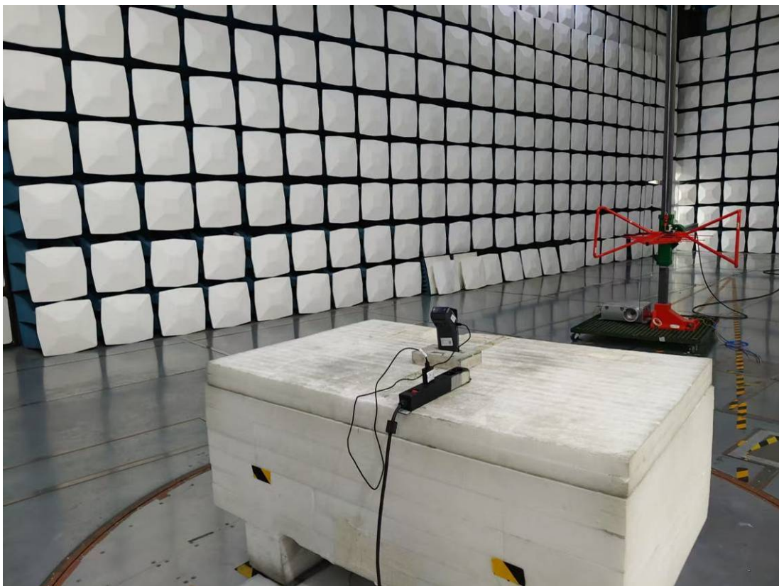
Radiated Emission 30M-1GHz View M1
