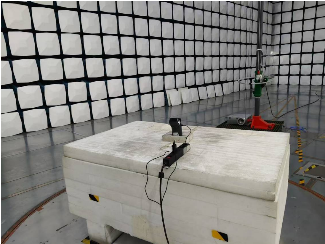
Radiated Emission 30M-1GHz View M2
