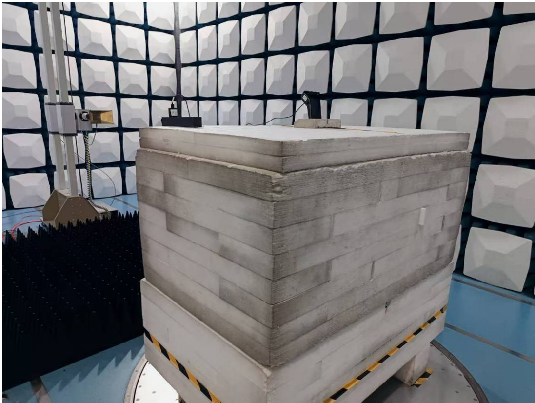
Radiated Emission 18-25GHz View M1
