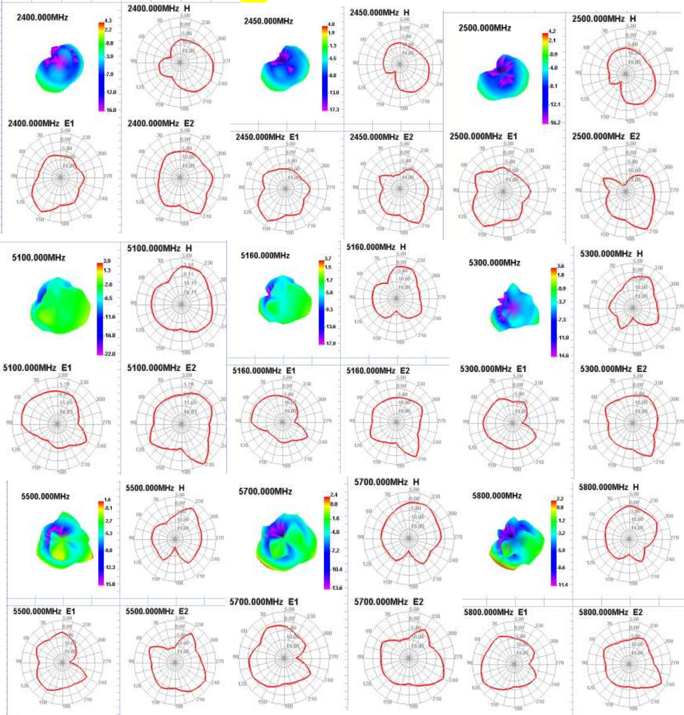
Directional pattern
