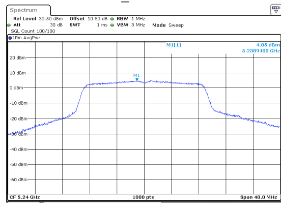
n20_5240MHz
