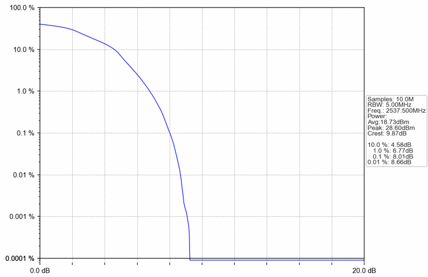
Band41_5MHz_16QAM_LCH_2537.5MHz_RB_25_0_NTNV
