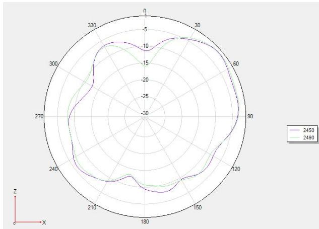
chart 1 Phi 0 2D
