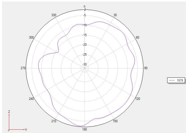
chart 3 Theta 90 2D
