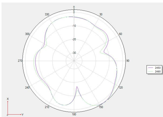
chart 3 Theta 90 2D
