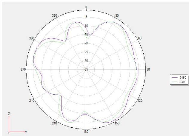
chart 2 Phi 90 2D
