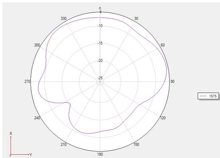
chart 3 Theta 90 2D
