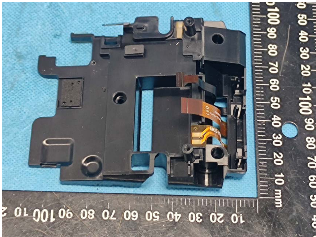
WiFi/Bluetooth Antenna
