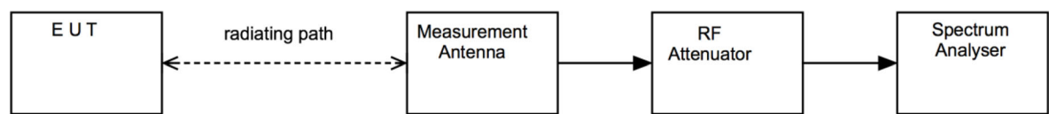
Figure i Test Setup
