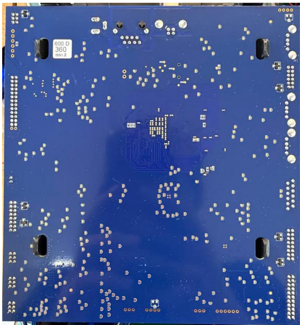
Figure 7: Bottom Side of Main PCB (PCB removed from product)
