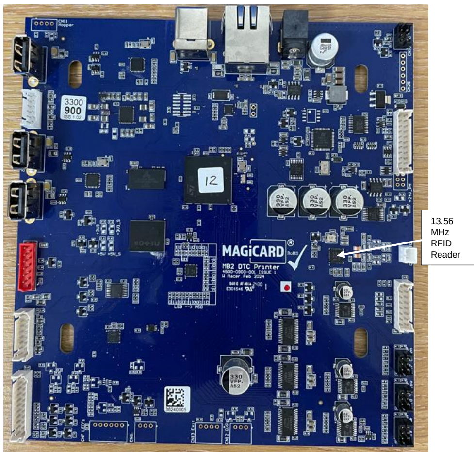
Figure 6: Top Side of Main PCB (PCB removed from product)
