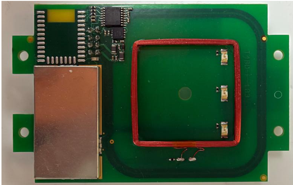
Figure 9: Underside of Elatec Smart Code Encoder PCB (PCB removed from product)
