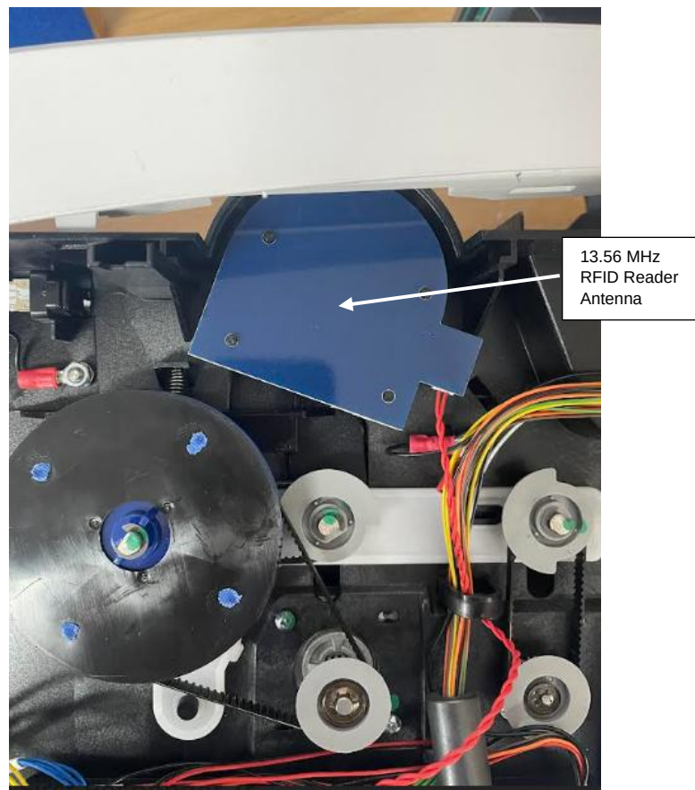
Figure 10: Close-Up view of view of RFID Antenna installed in product
