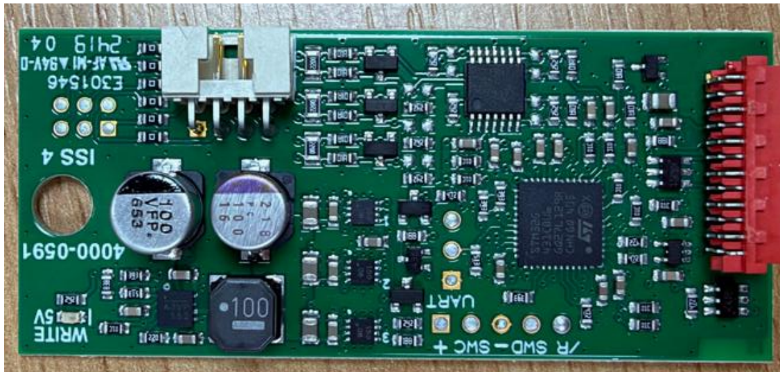
Figure 12: Top side of Mag Encoder PCB (PCB removed from product)
