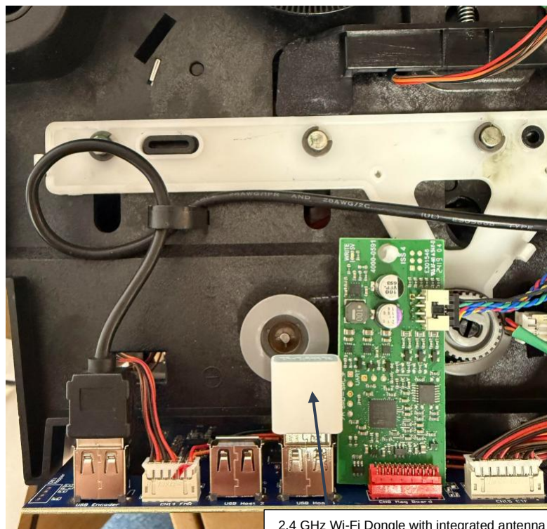
2.4 GHz Wi-Fi Dongle with integrated antenna
