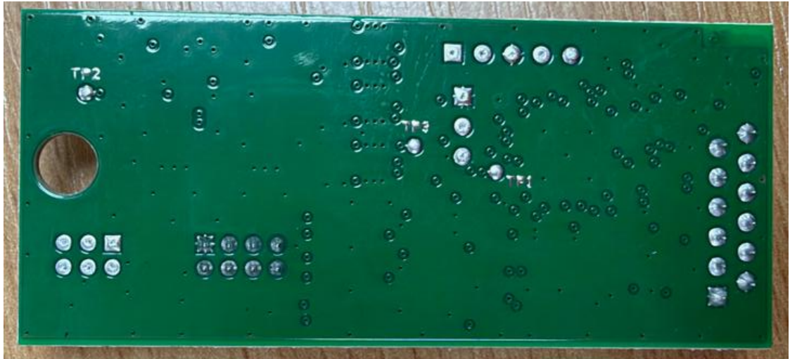
Figure 13: Underside of Mag Encoder PCB (PCB removed from product)
