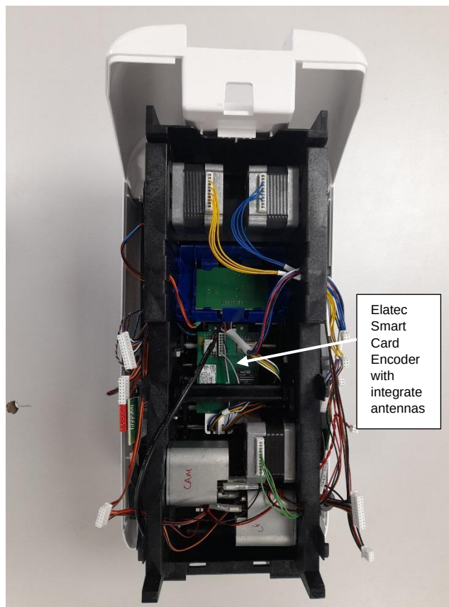
Figure 4: Underside (main PCB removed)
