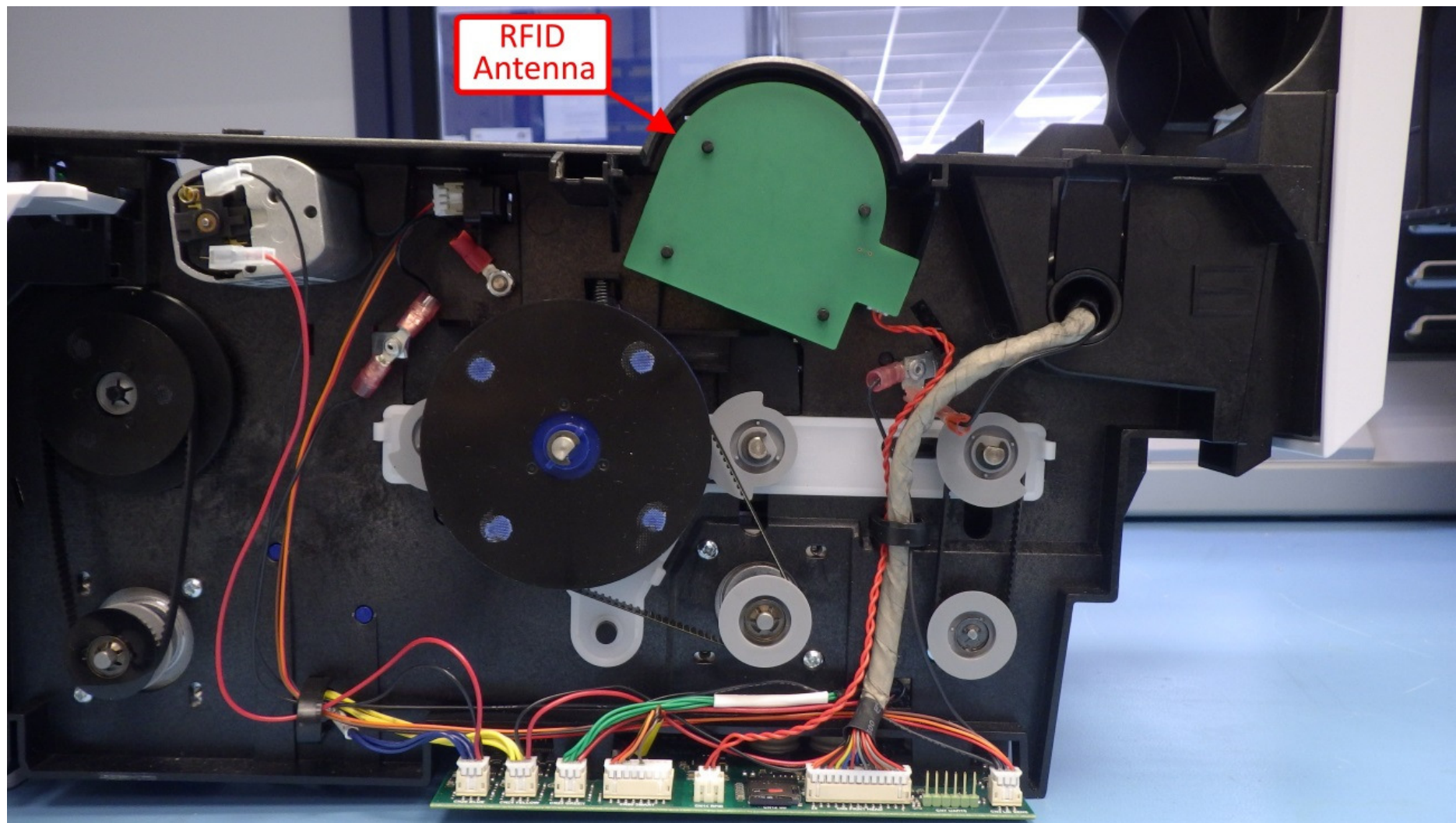
Right side with antenna PCB visible and highlighted
