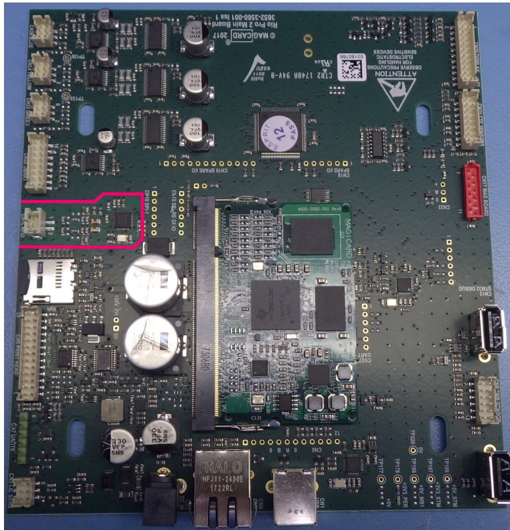
Main PCB – RF circuitry highlighted
