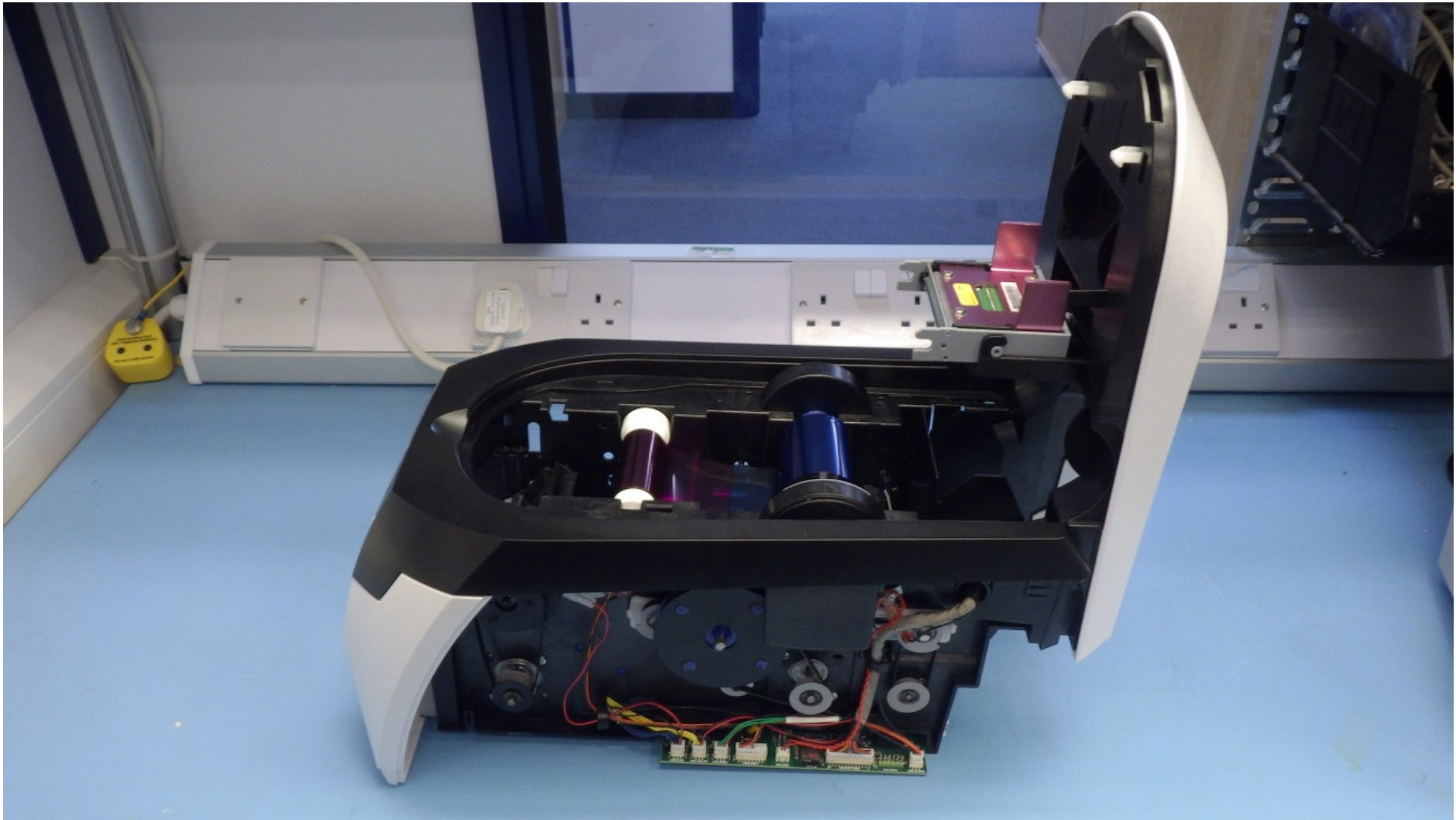
Right side viewed from above with lid open
