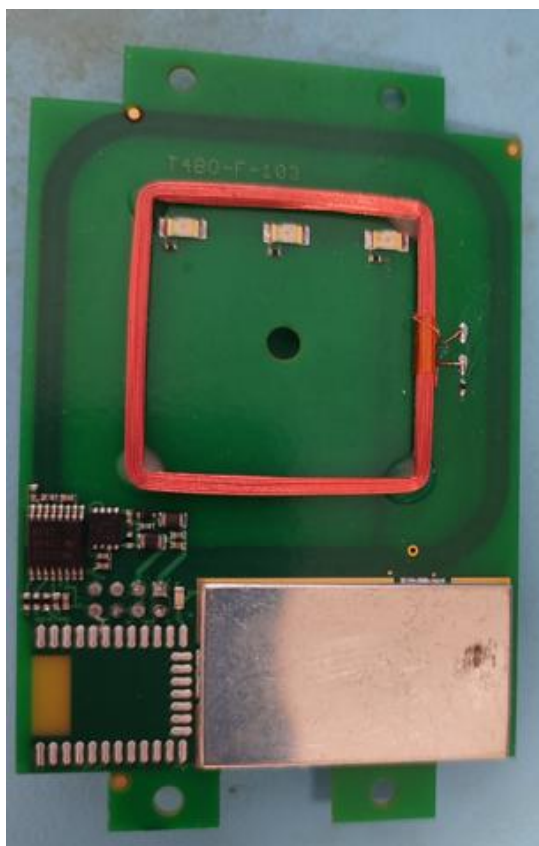
13.56 MHz RFID Board
