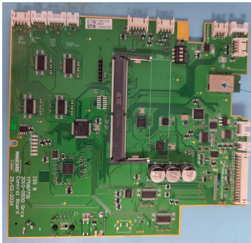
Control Board – Bottom
