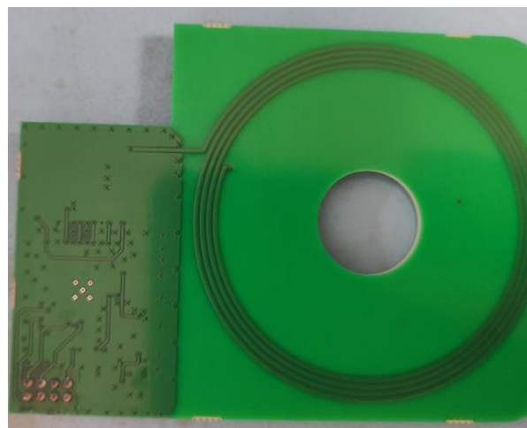
13.56 MHz RFID Board
