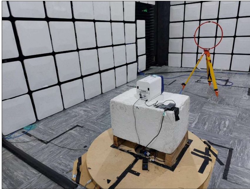
Figure 15 - Test Setup – 9 kHz to 30 MHz
