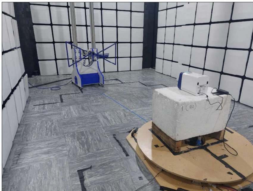
Figure 16 - Test Setup –30 MHz to 1 GHz
