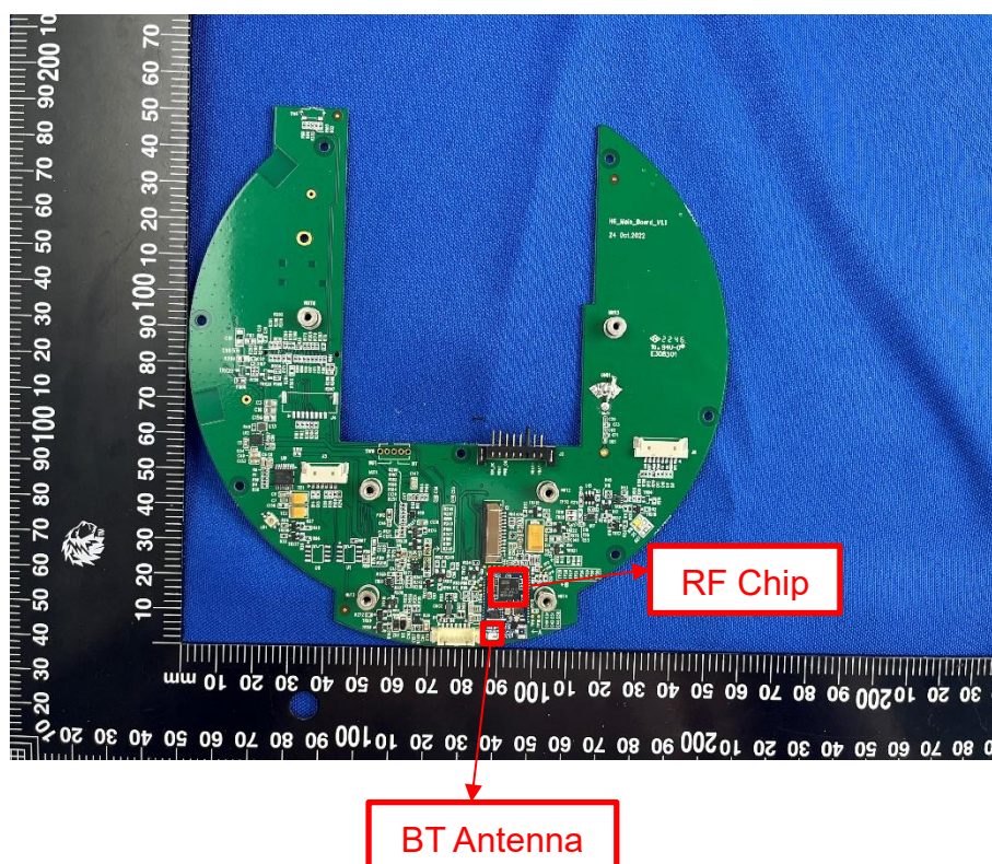
MAIN BOARD TOP VIEW (WITHOUT SHIELDING)
