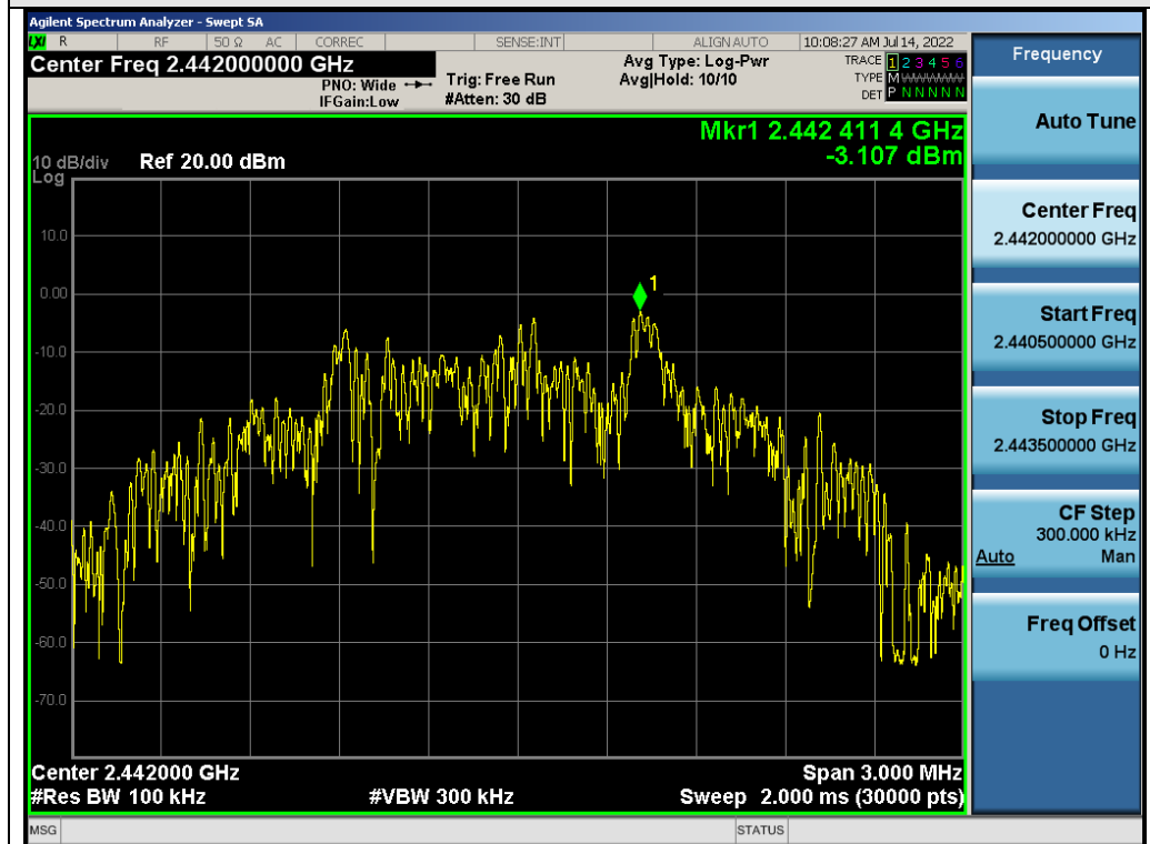
Test_Graph_2.4G_ANT1_2442_Reference Level
