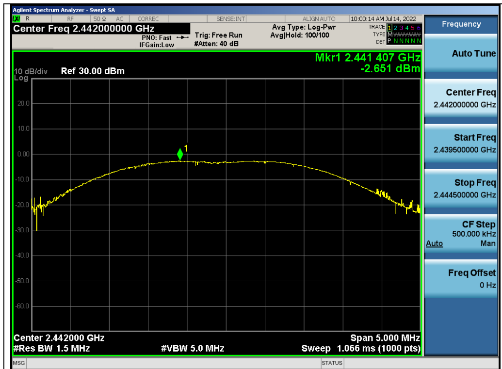
Test_Graph_2.4G_ANT1_2442_Peak Power
