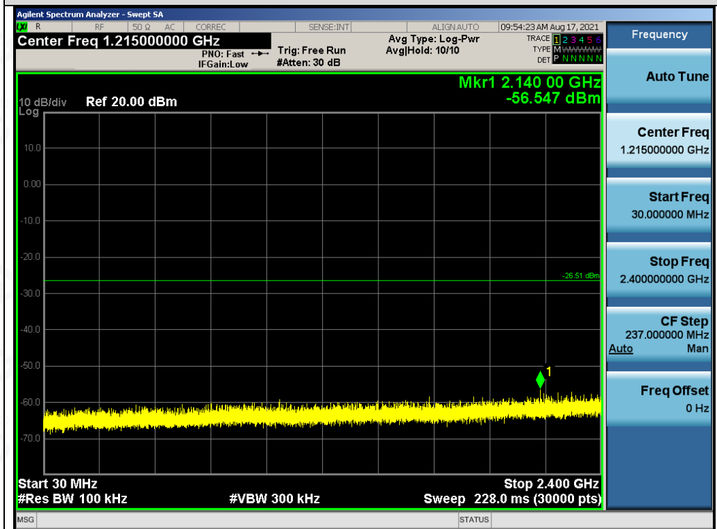
Test_Graph_GFSK_ANT1_2475_2Mbps_Lower Band Emissions
