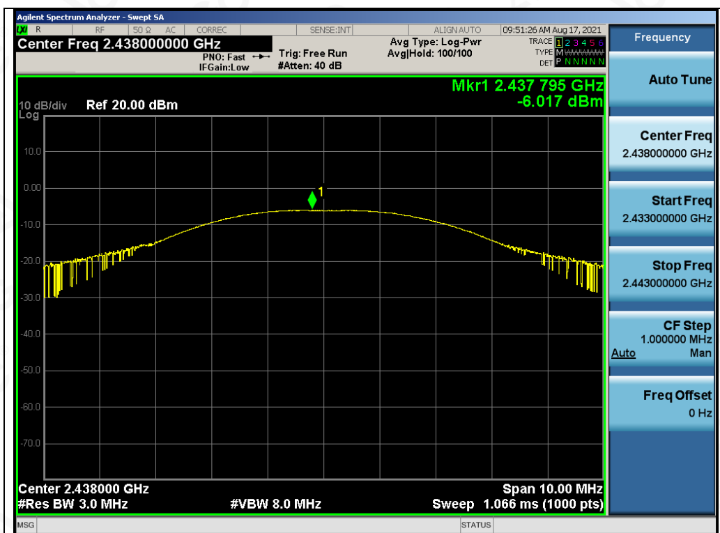
Test_Graph_GFSK_ANT1_2438_2Mbps_Peak Power
