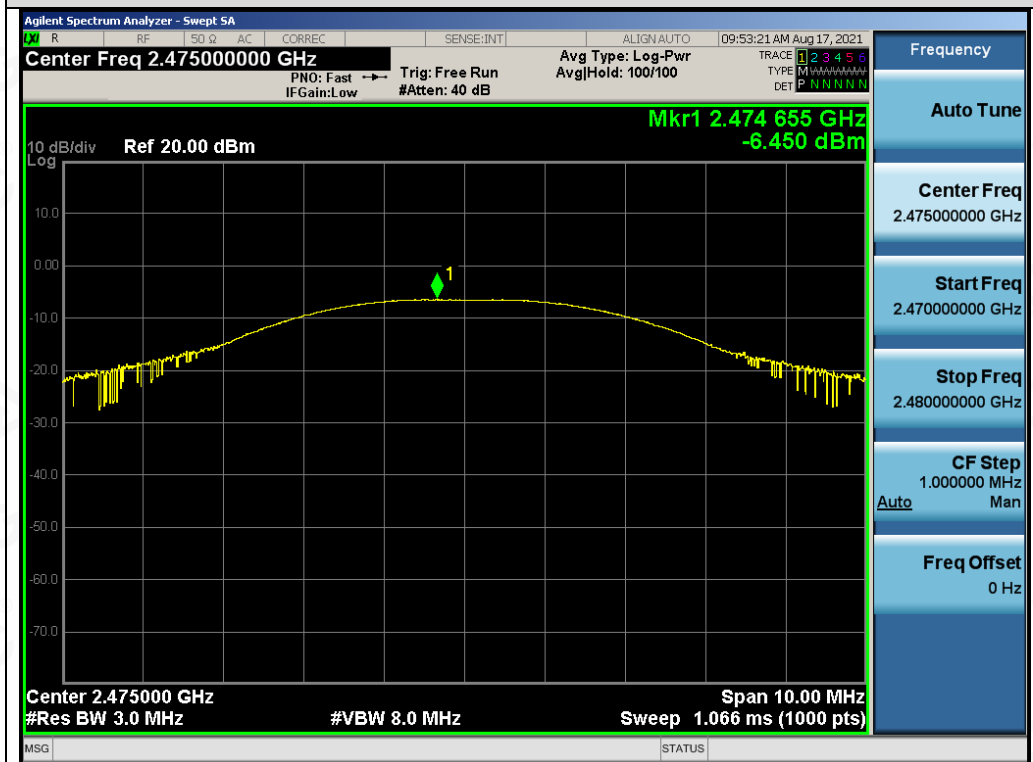
Test_Graph_GFSK_ANT1_2475_2Mbps_Peak Power
