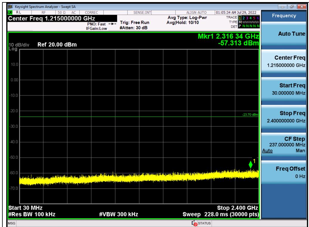
Test_Graph_2.4G_ANT1_2442_Lower Band Emissions
