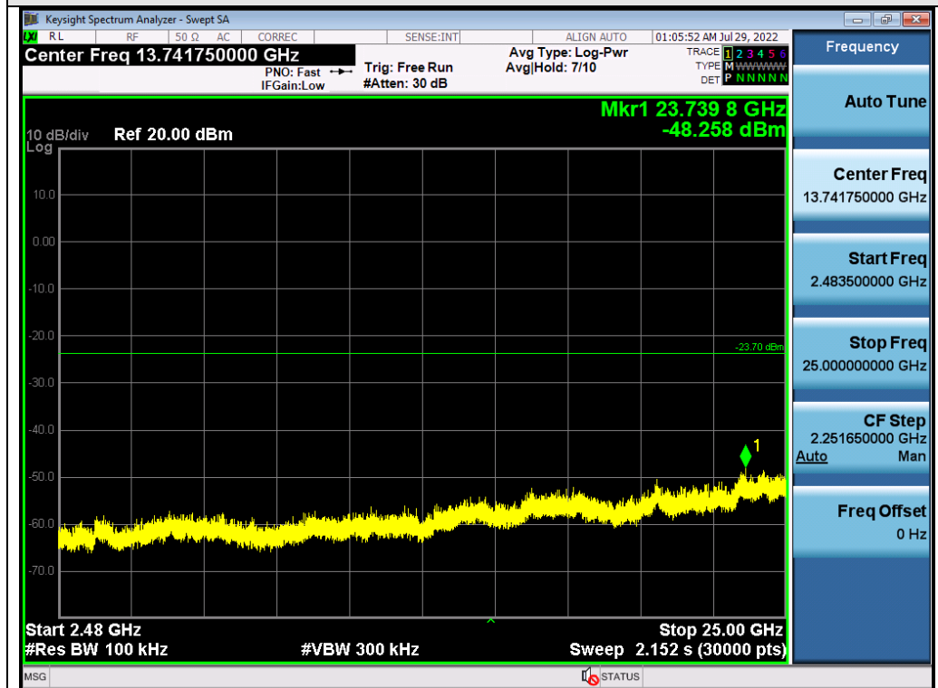
Test_Graph_2.4G_ANT1_2442_Higher Band Emissions
