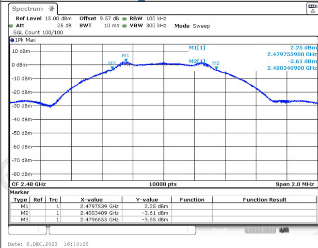
LE_Channel 39
