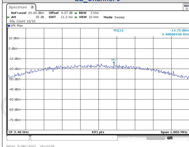
LE_Channel 39
