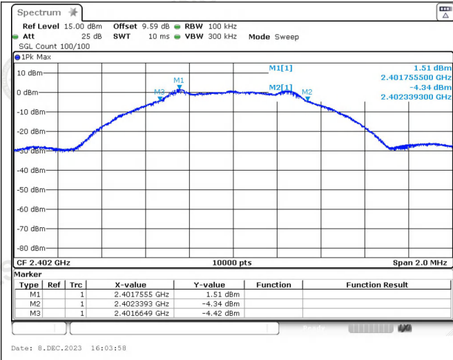
LE_Channel 0
