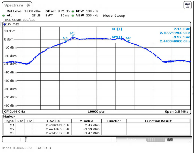
LE_Channel 19
