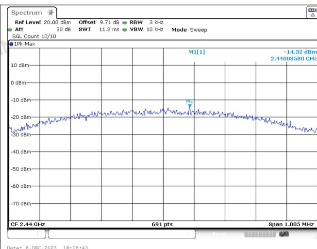
LE_Channel 19
