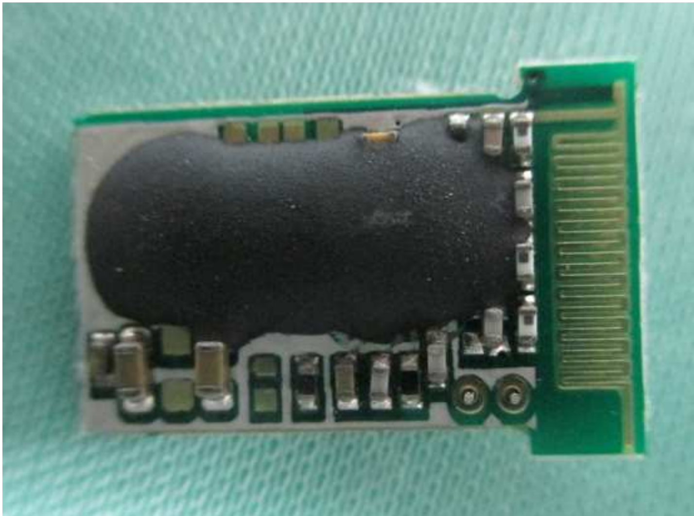
FCC ID: XENG001 PHOTOGRAPH OF THE PRODUCT INNER CIRCUIT TOP VIEW
