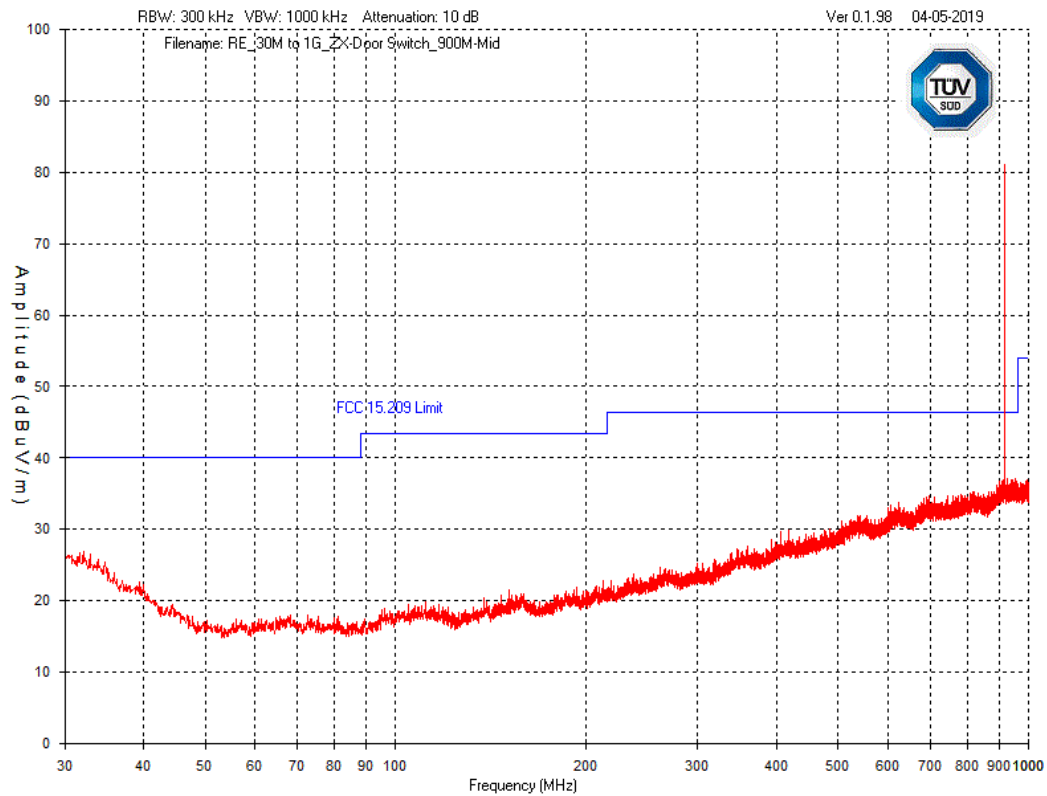
Graph 19 Test Results – Tx Spurious Emission 30MHz to 1GHz – Mid Channel – Vertical Polarization
