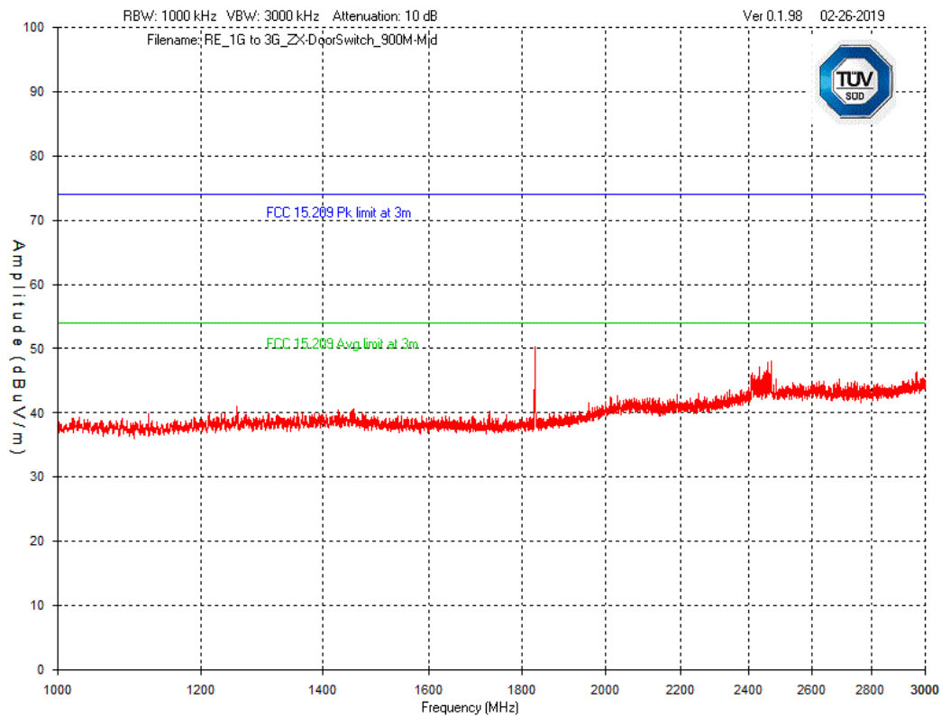
Graph 21 Test Results – Tx Spurious emission 1GHz to 3GHz – Mid Channel – Vertical Polarization
