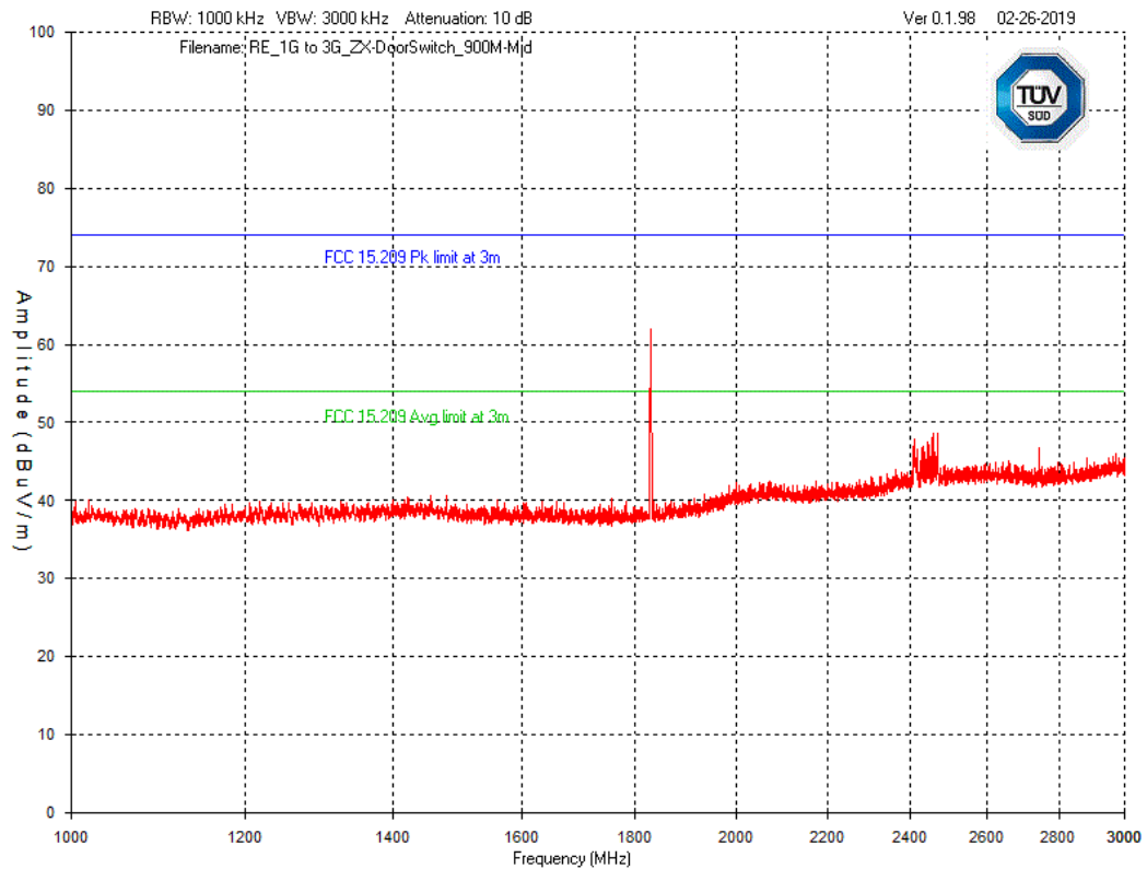
Graph 22 Test Results – Tx Spurious emission 1GHz – 3GHz – Mid Channel – Horizontal Polarization
