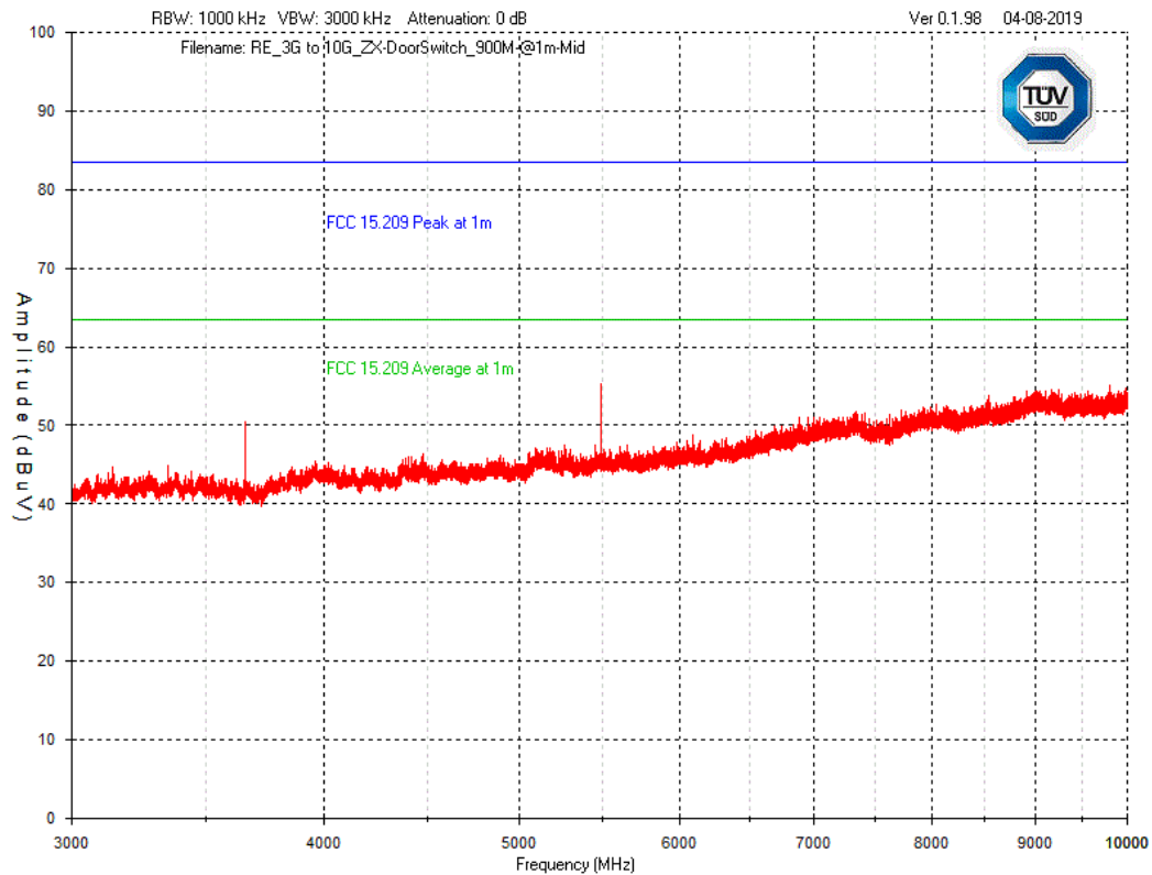
Graph 24 Test Results – Tx Spurious emission 3GHz – 10GHz – Mid Channel – Vertical polarisation
