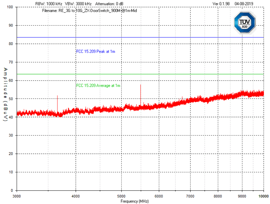
Graph 23 Test Results – Tx Spurious emission 3GHz – 10GHz – Mid Channel – Horizontal Polarization
