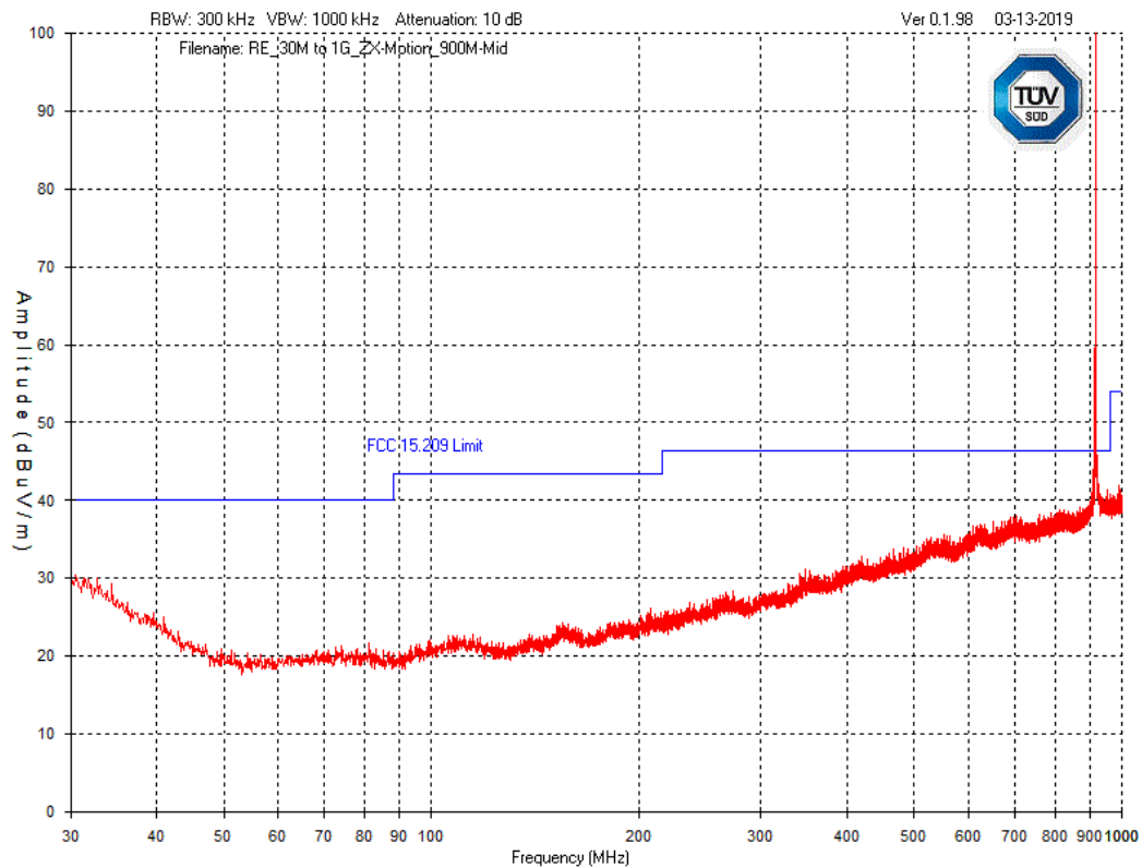
Graph 21 Test Results – Tx Spurious emission 30MHz to 1GHz – Mid Channel – Horizontal Polarization
