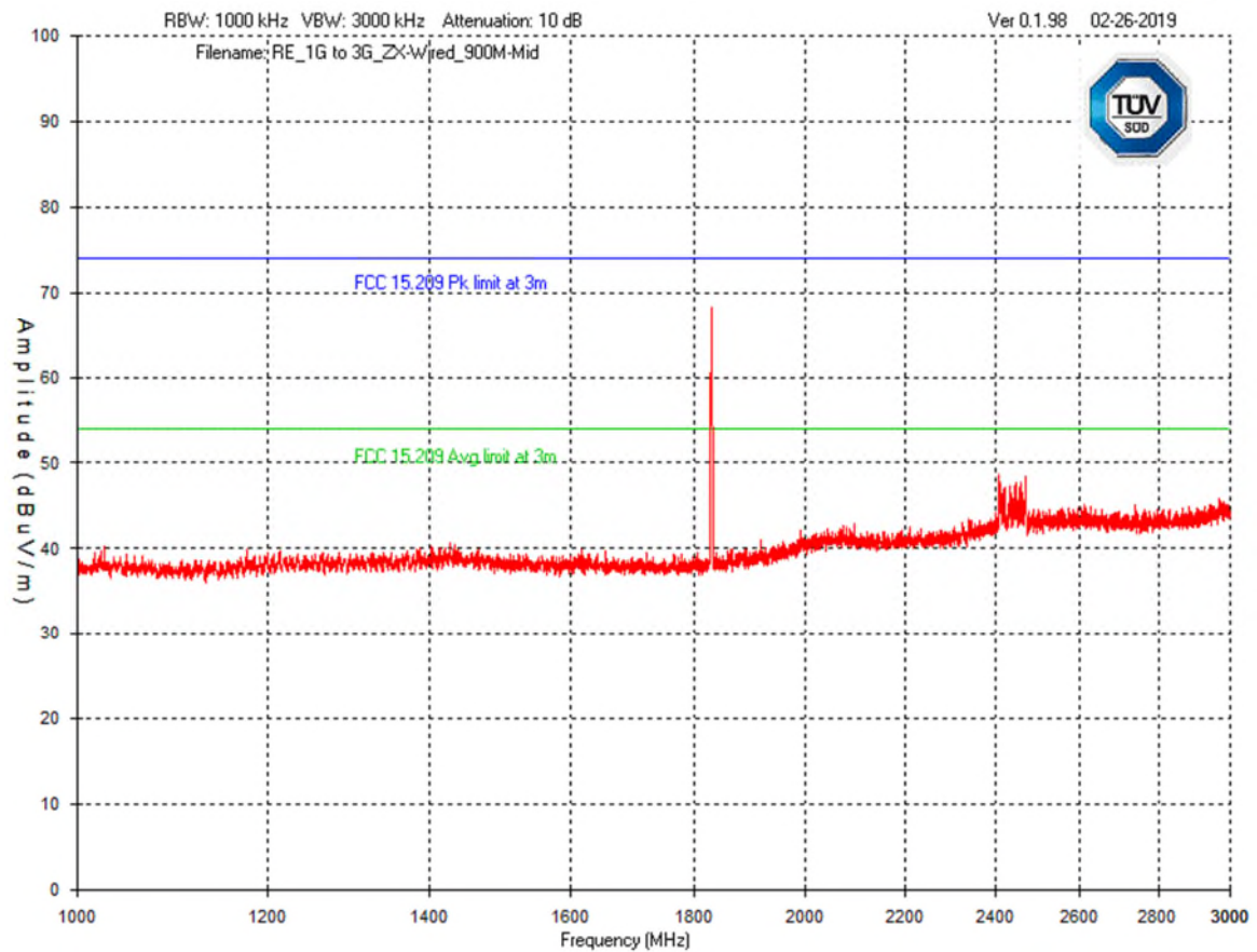
Graph 43 Test Results – Tx Spurious emission 1GHz – 3GHz-(Horizontal polarisation): Mid Channel ZX Wired Thermostat (900MHz)
