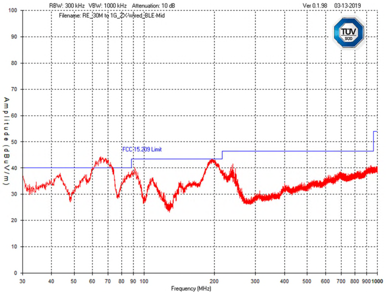
Graph 39 Test Results – Tx Spurious emission 30MHz – 1GHz (Vertical polarisation): Mid Channel ZX Wired Thermostat (2.4GHz)
