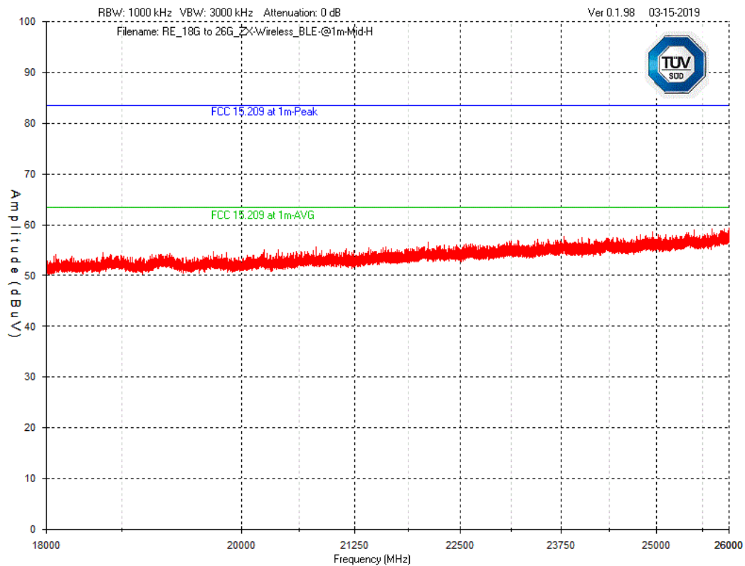
Graph 55 Test Results – Tx Spurious emission 18GHz – 26GHz: Mid Channel ZX Wireless Thermostat (2.4GHz) – Horizontal Polarization
