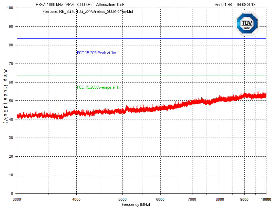
Graph 49 Test Results – Tx Spurious emission 3GHz – 10GHz: Mid Channel ZX Wireless Thermostat (900MHz) – Horizontal Polarization
