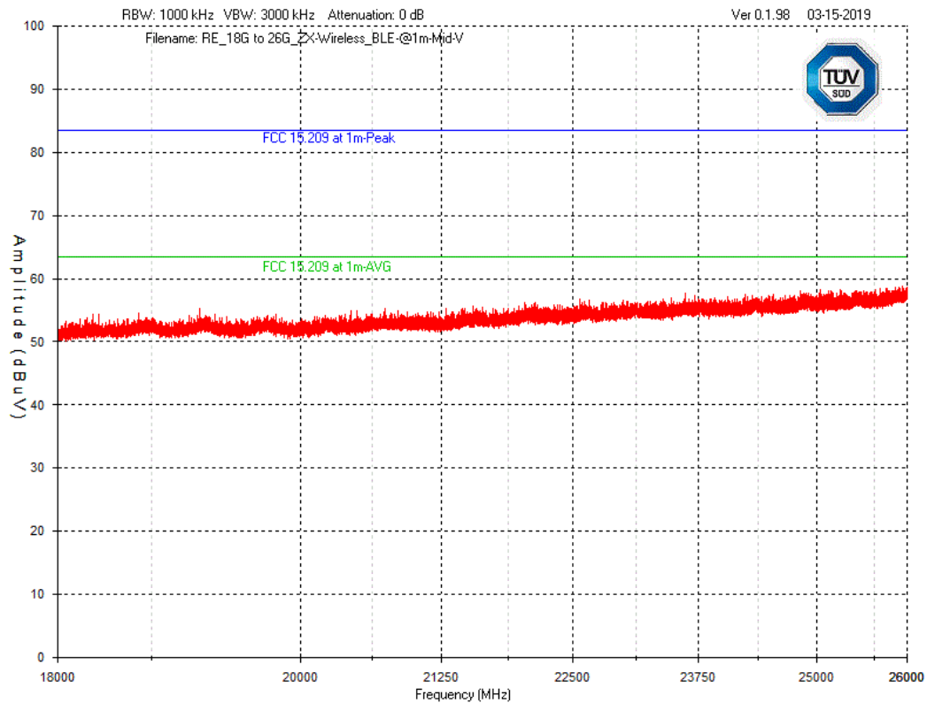
Graph 56 Test Results – Tx Spurious emission 18GHz – 26GHz: Mid Channel ZX Wireless Thermostat (2.4GHz) – Vertical Polarization
