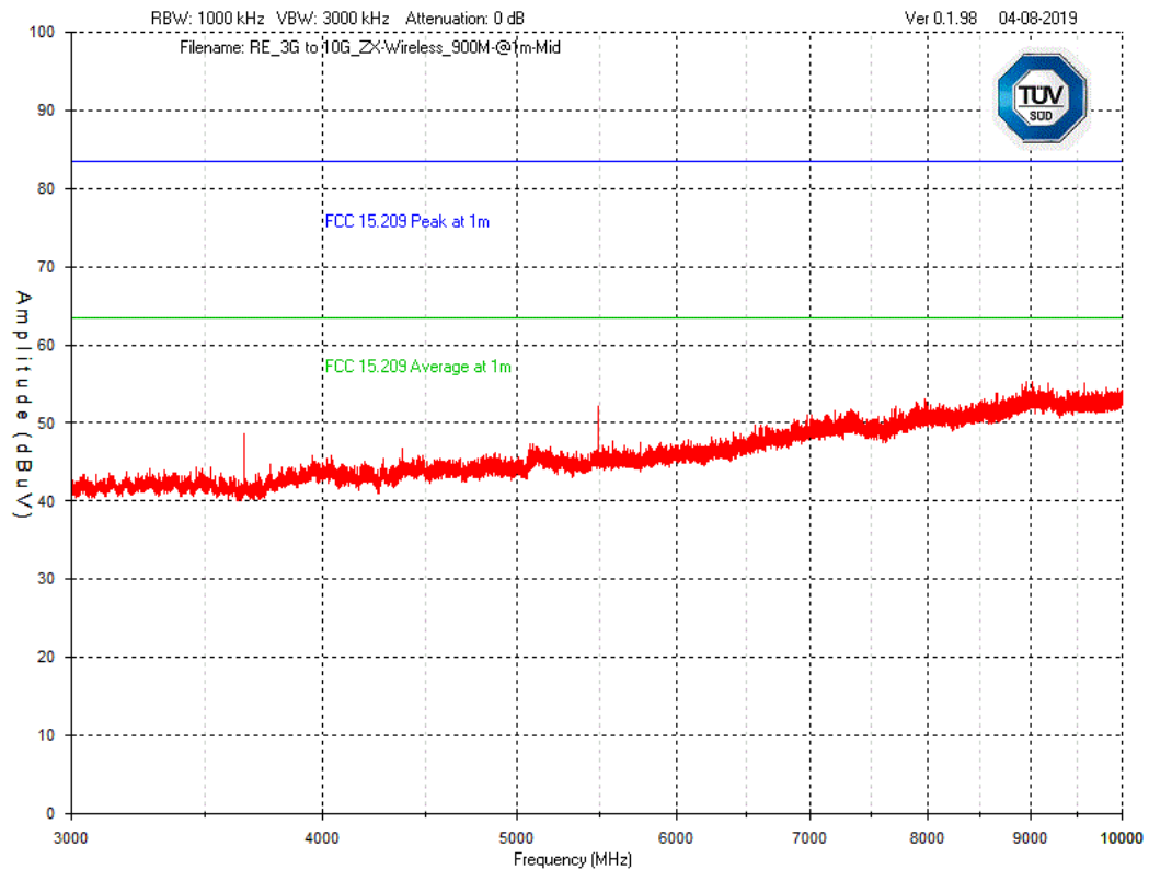
Graph 50 Test Results – Tx Spurious emission 3GHz – 10GHz: Mid Channel ZX Wireless Thermostat (900MHz) – Vertical Polarization
