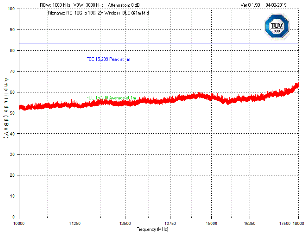
Graph 53 Test Results – Tx Spurious emission 10GHz – 18GHz: Mid Channel ZX Wireless Thermostat (2.4GHz) – Horizontal Polarization
