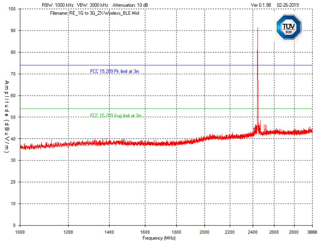
Graph 48 Test Results – Tx Spurious emission 1GHz – 3GHz: Mid Channel ZX Wireless Thermostat (2.4GHz) – Vertical Polarization
