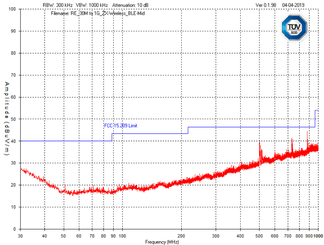
Graph 42 Test Results – Tx Spurious emission 30MHz – 1GHz: Mid Channel ZX Wireless Thermostat(2.4GHz) – Vertical Polarization
