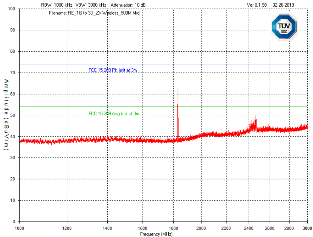
Graph 46 Test Results – Tx Spurious emission 1GHz – 3GHz: Mid Channel ZX Wireless Thermostat (900MHz) – Horizontal Polarization
