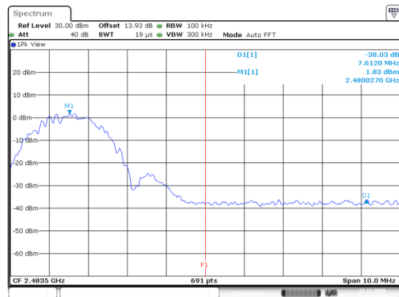
BLE-2M High CH
