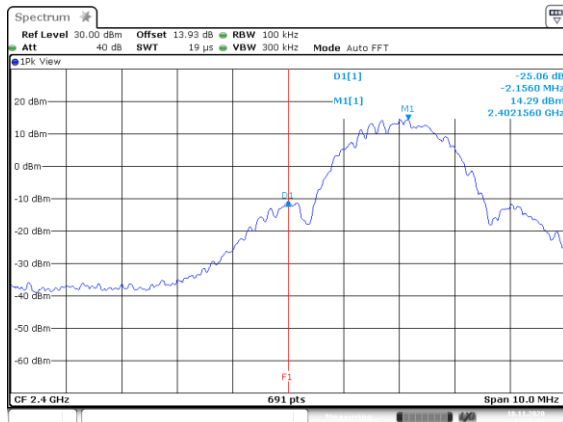
BLE-2M Low CH
