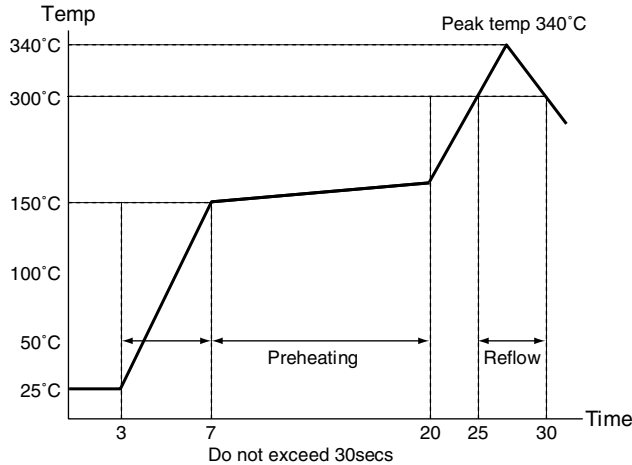
MAXIMUM REFLOW SOLDERING PROFILE
