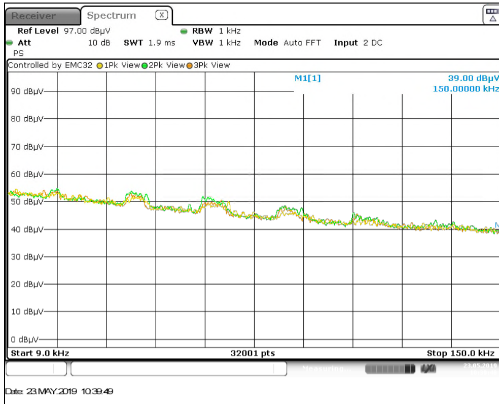
Figure A-3: Radiated Emissions – 9kHz-150kHz
