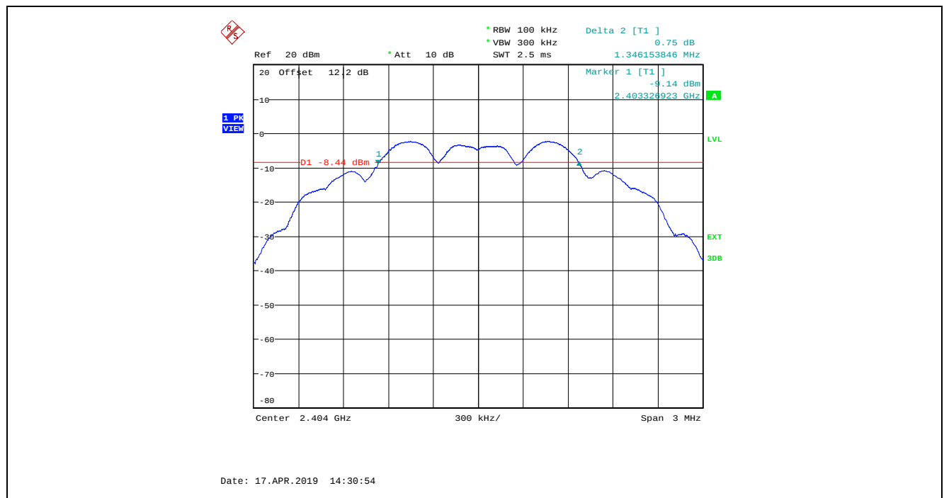
Plot 5.2.4.4. 6 dB Bandwidth, GFSK Modulation, Power Setting at 15, Channel 00, 2404 MHz, 2 Mbps
