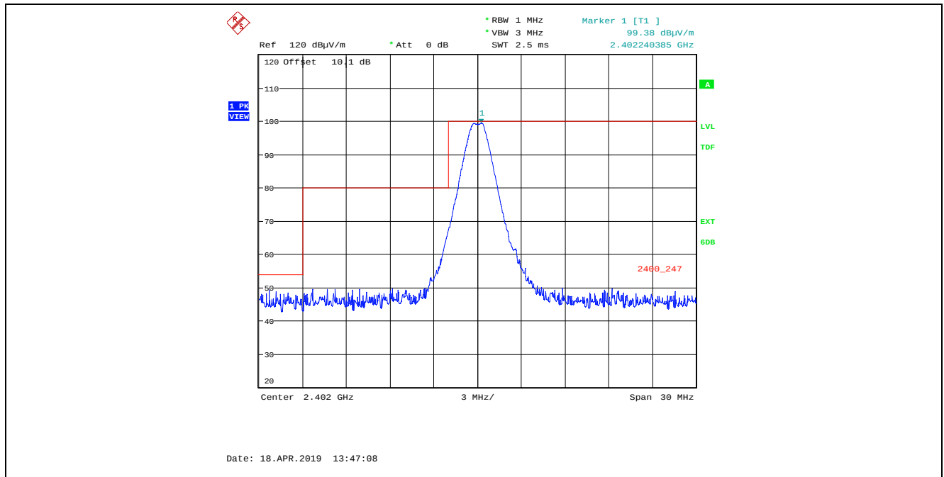
Plot 5.4.4.2.1. Band-Edge Radiated Emissions, Lower Band-edge Rx Antenna in Vertical Polarization, GFSK Modulation, 1 Mbps, Power Setting 15, Ch 37, 2402 MHz
