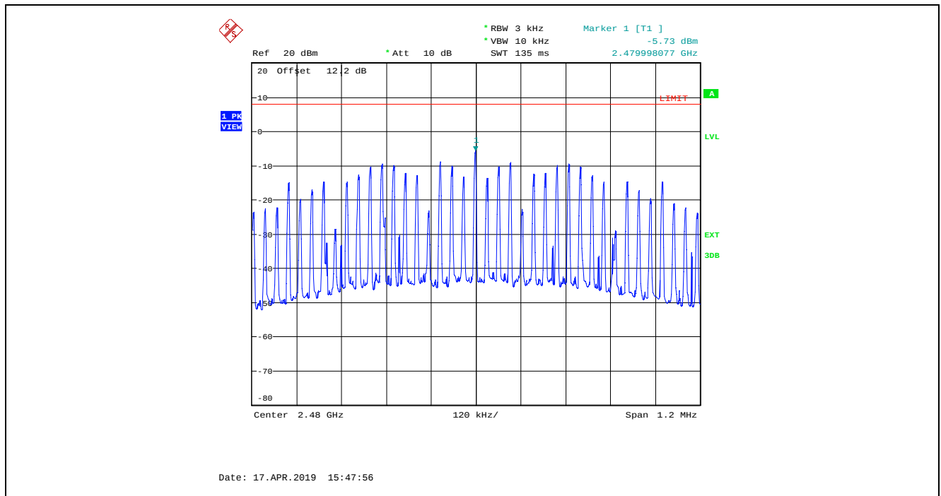
Plot 5.5.4.3. Power Spectral Density, GFSK Modulation, 1 Mbps, Power Setting 15, Channel 39, 2480 MHz
