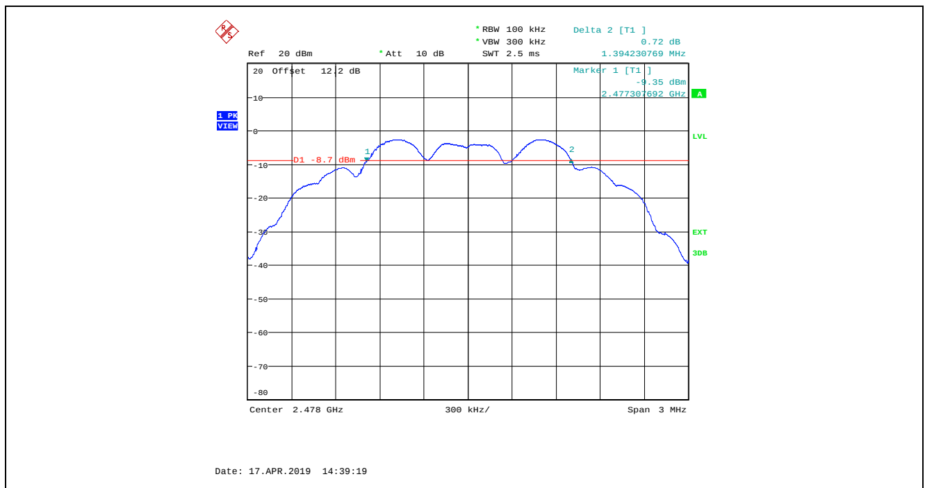
Plot 5.2.4.6. 6 dB Bandwidth, GFSK Modulation, Power Setting at 15, Channel 36, 2478 MHz, 2 Mbps
