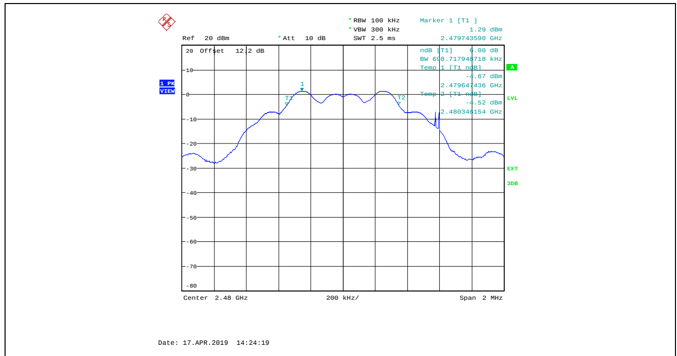
Plot 5.2.4.3. 6 dB Bandwidth, GFSK Modulation, Power Setting at 15, Channel 39, 2480 MHz, 1 Mbps
