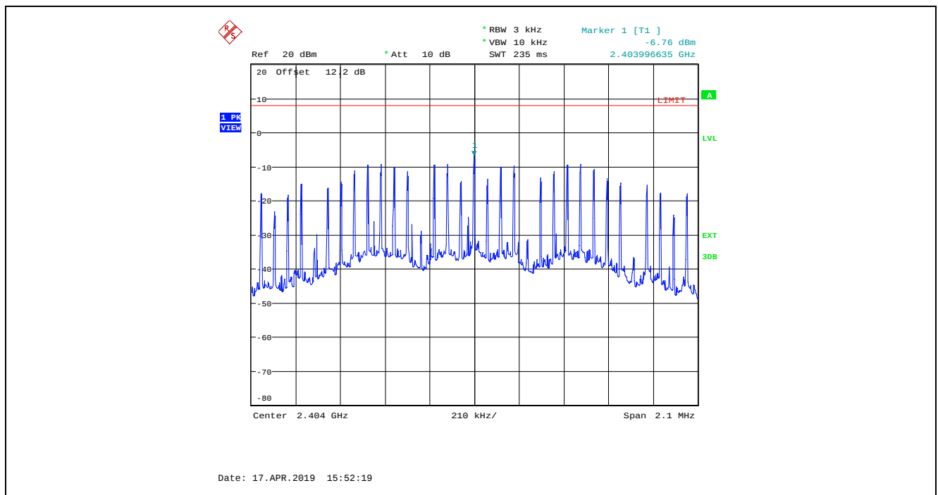
Plot 5.5.4.4. Power Spectral Density, GFSK Modulation, 2 Mbps, Power Setting 15, Channel 00, 2404 MHz
