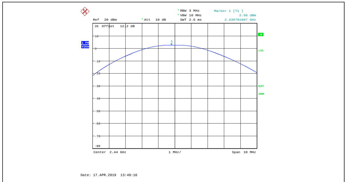
Plot 5.3.4.2. Maximum Peak Conducted Output Power, GFSK Modulation, 1 Mbps, Power Setting 15, Ch 17, 2440 MHz
