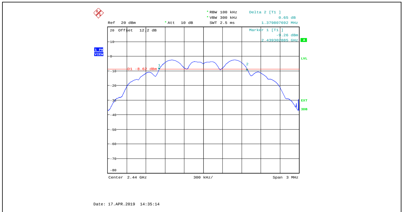
Plot 5.2.4.5. 6 dB Bandwidth, GFSK Modulation, Power Setting at 15, Channel 17, 2440 MHz, 2 Mbps
