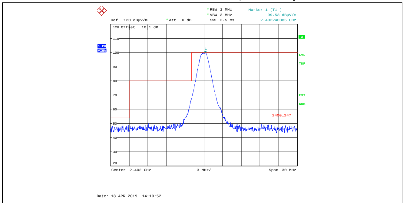
Plot 5.4.4.2.2. Band-Edge Radiated Emissions, Lower Band-edge Rx Antenna in Horizontal Polarization, GFSK Modulation, 1 Mbps, Power Setting 15, Ch 37, 2402 MHz
