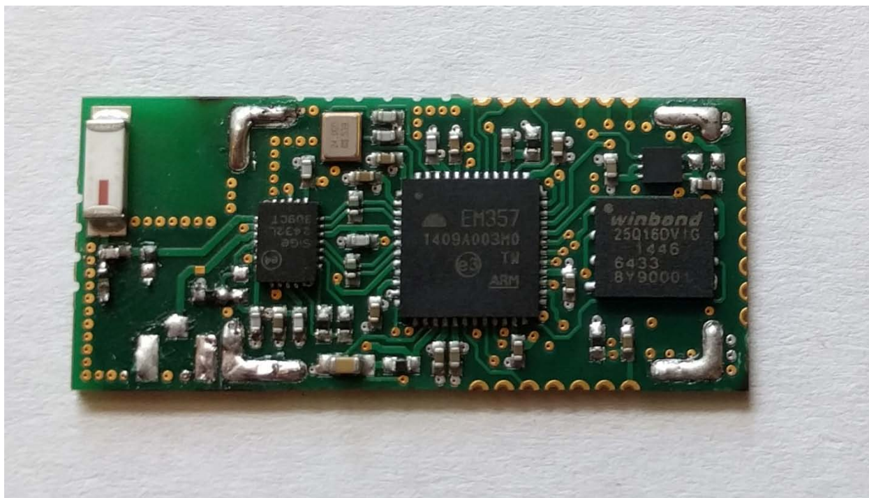
Figure 1: EUT Internal photo – top view
