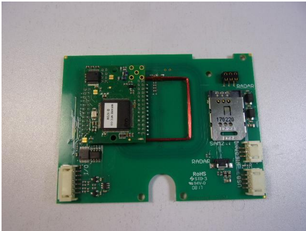
PCR-TWN4 rear side
