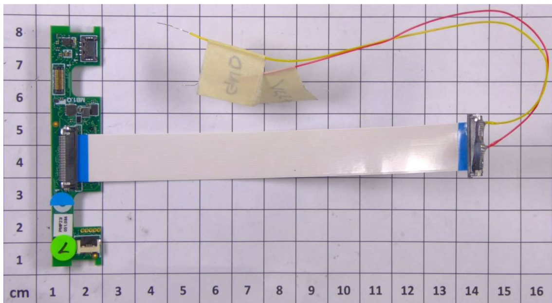
(EUT with attached custom-built power supply cable)
