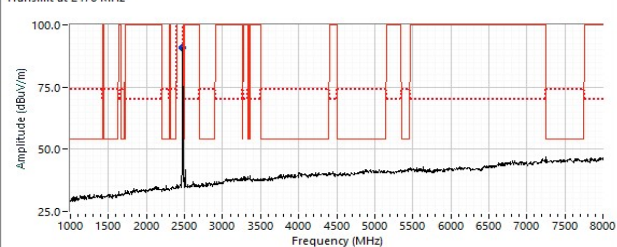
Transmit at 2476 MHz
