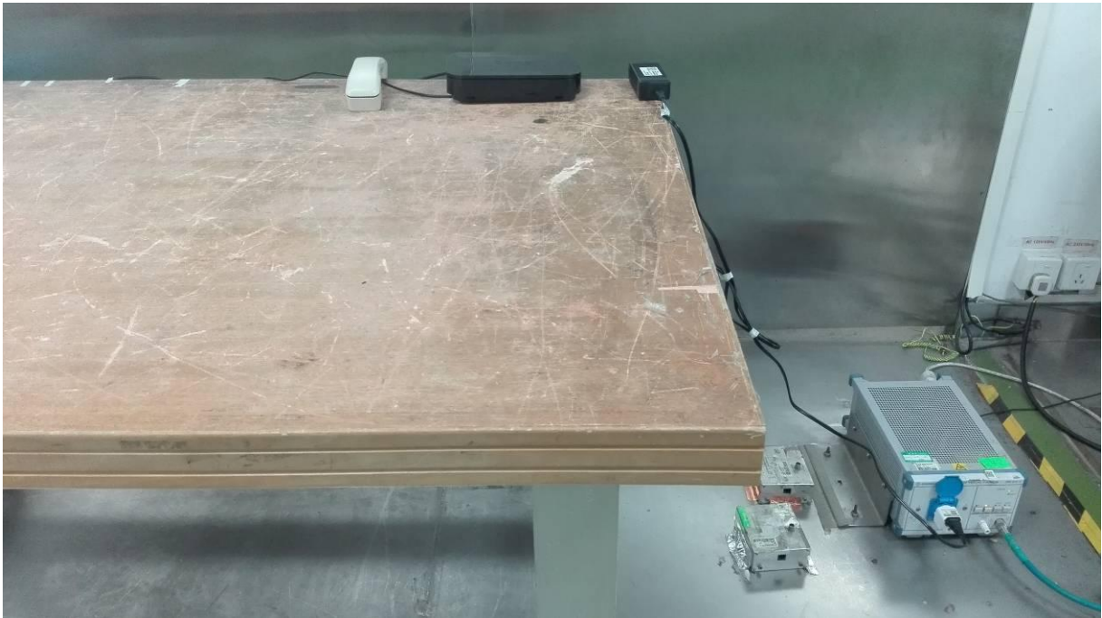
Conducted Emissions - Front View
