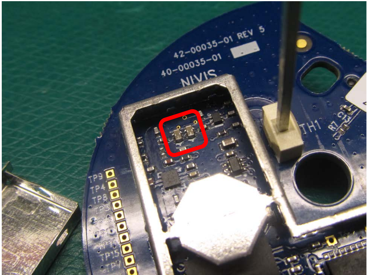
Modification indicated: changed filter components boxed in red.
