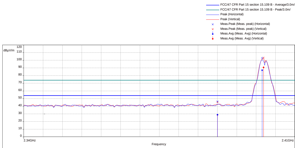
Figure 39: Band-edge-2402 MHz
