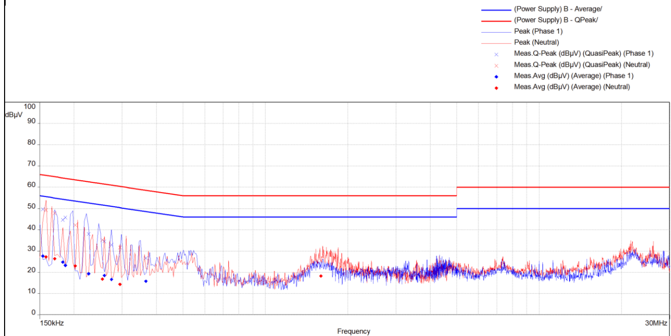
150 kHz to 30 MHz Plot for Live and Neutral
