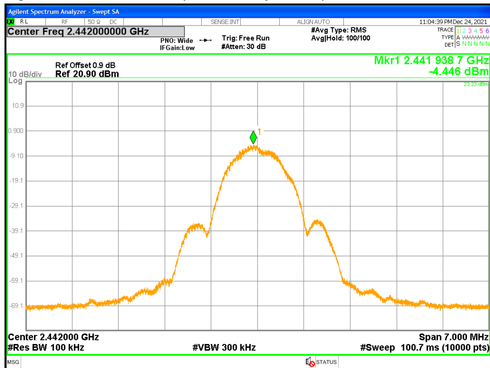
Figure 22: Maximum Power Spectral Density at 1 Mbps - 2442 MHz - Transmitter
