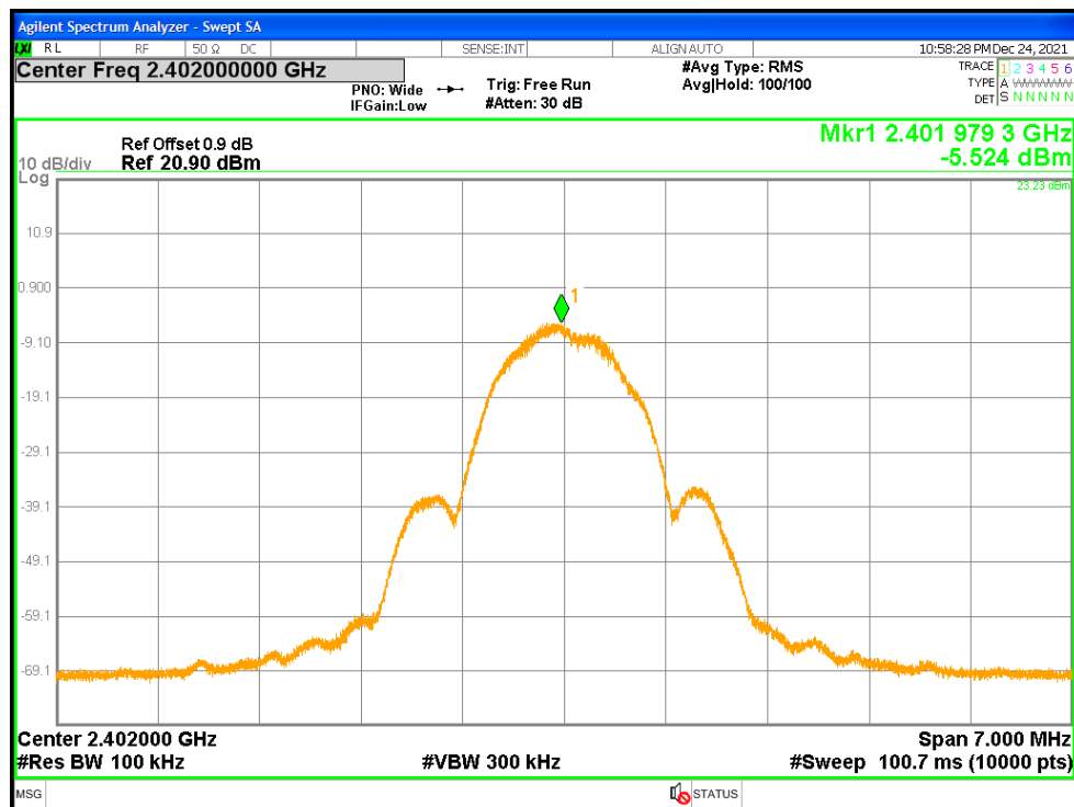
Figure 21: Maximum Power Spectral Density at 1 Mbps - 2402 MHz - Transmitter
