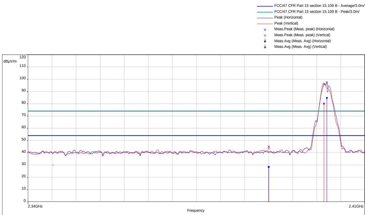
Figure 39: Band-edge-2402 MHz
