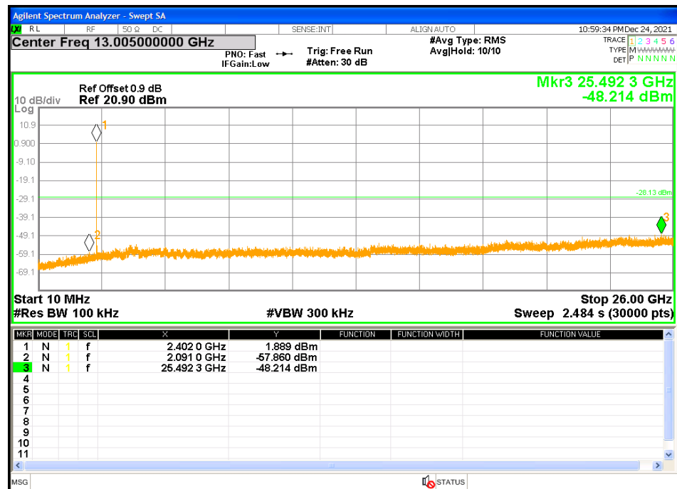
Figure 28: Out of band Emissions at 1 Mbps, 2402 MHz- Transmitter
