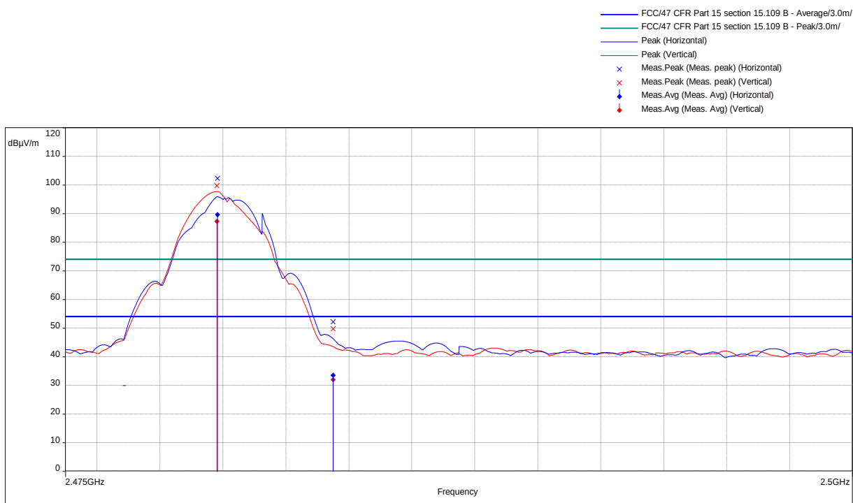
Figure 40: Band-edge-2480 MHz
