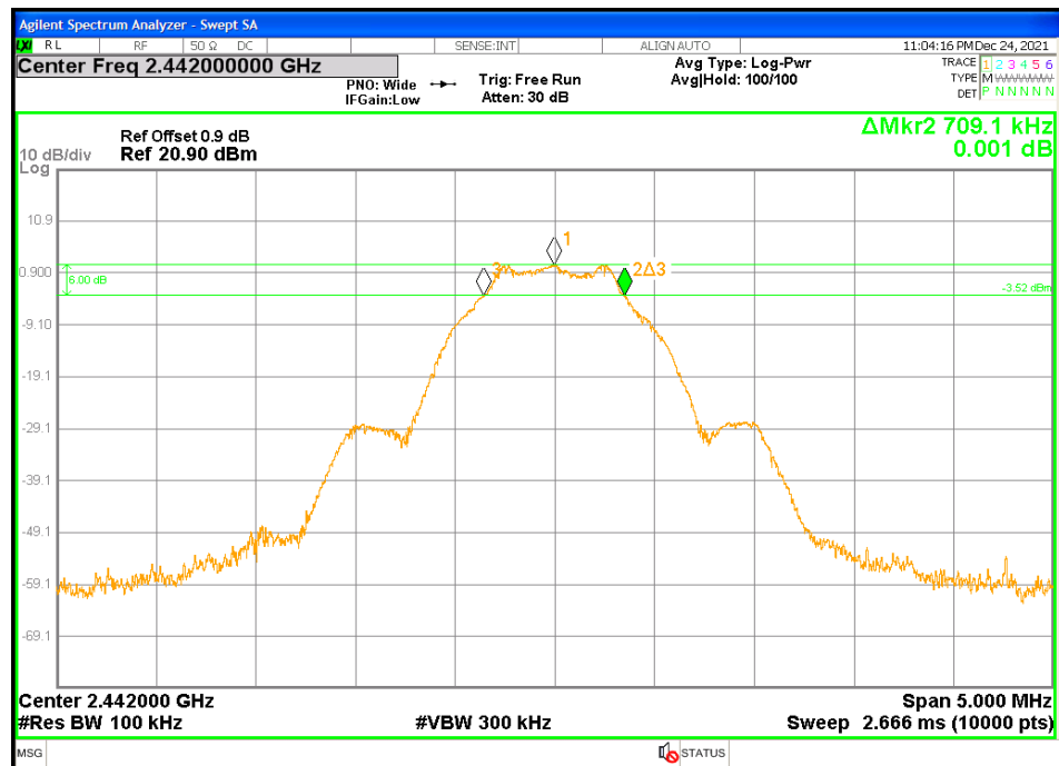
Figure 10: DTS Bandwidth - Transmitter at 1 Mbps - 2442 MHz
