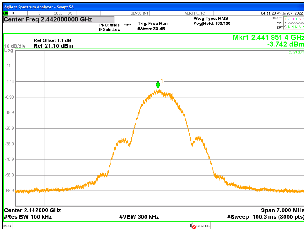
Figure 22: Maximum Power Spectral Density at 1Mbps - 2442 MHz - Headset
