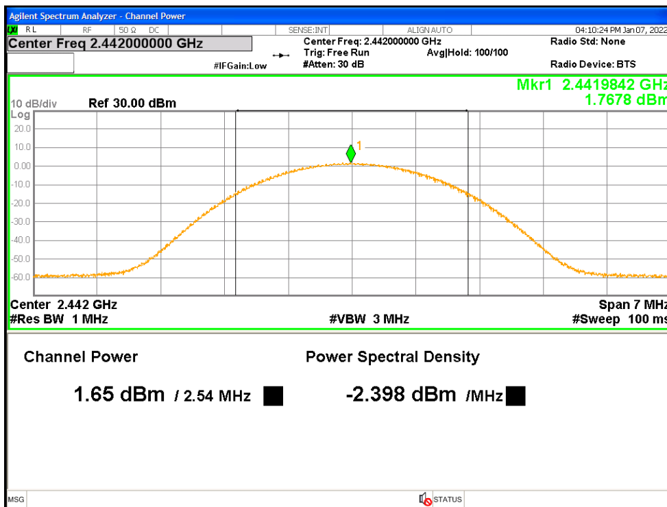
Figure 4: Maximum Conducted Output Power at 1Mbps, 2442 MHz - Headset
