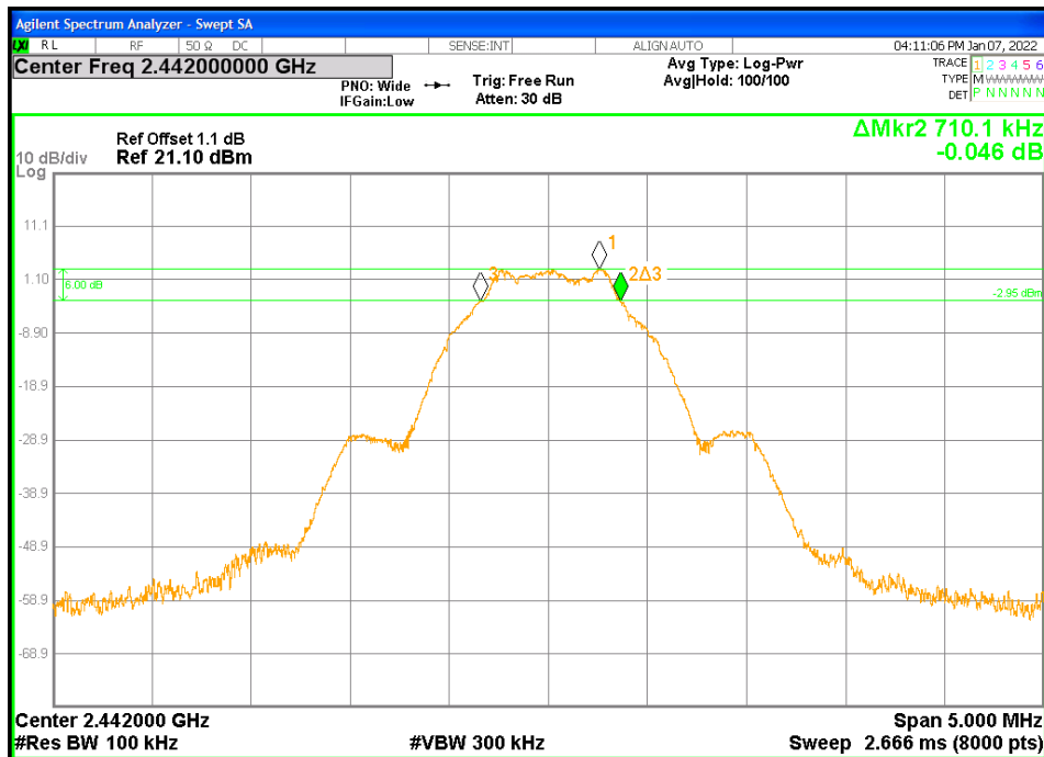
Figure 10: DTS Bandwidth-Headset at 1Mbps - 2442 MHz
