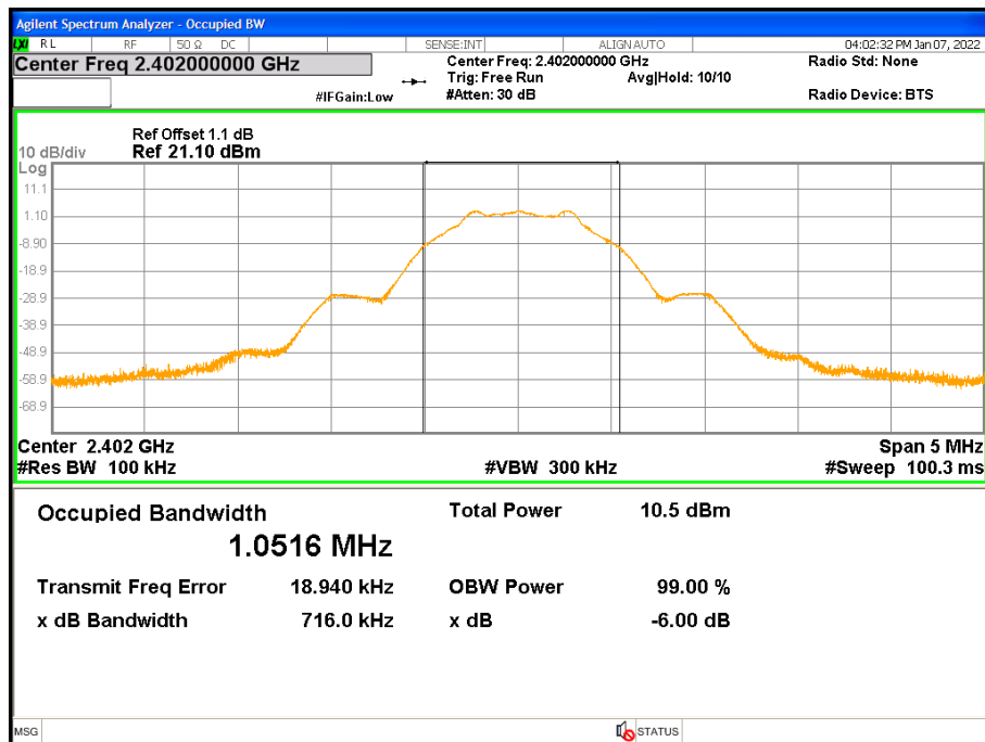
Figure 12: 99% Bandwidth-Headset at 1Mbps - 2402 MHz
