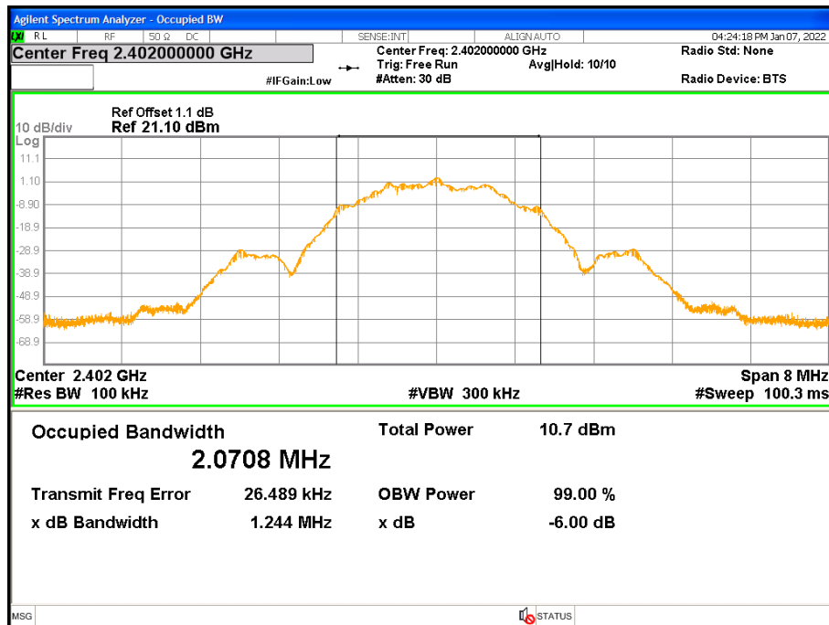
Figure 18: 99% Bandwidth-Headset at 2Mbps - 2402 MHz
