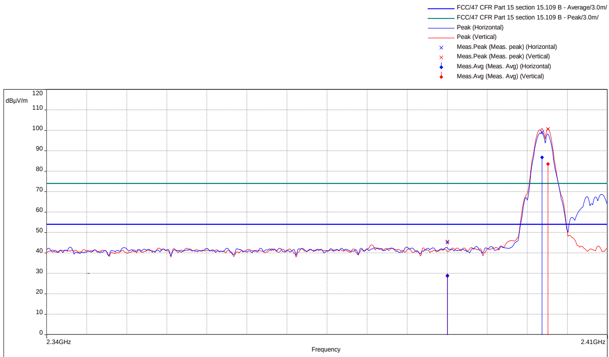
Figure 39: Band-edge-2402 MHz
