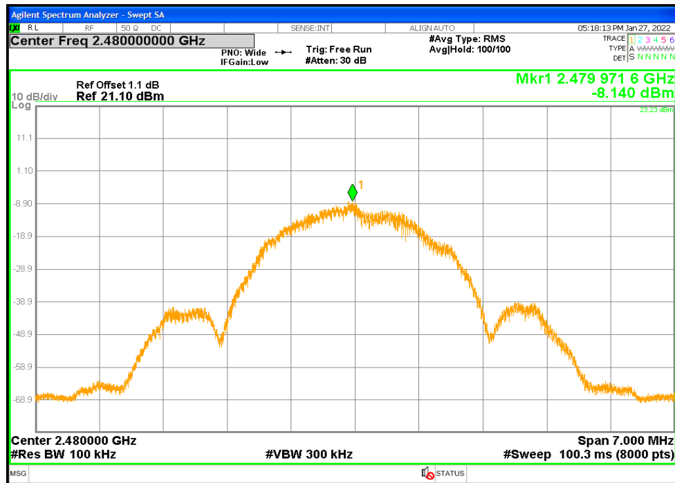
Figure 26: Maximum Power Spectral Density at 2 Mbps - 2480 MHz - Transmitter
