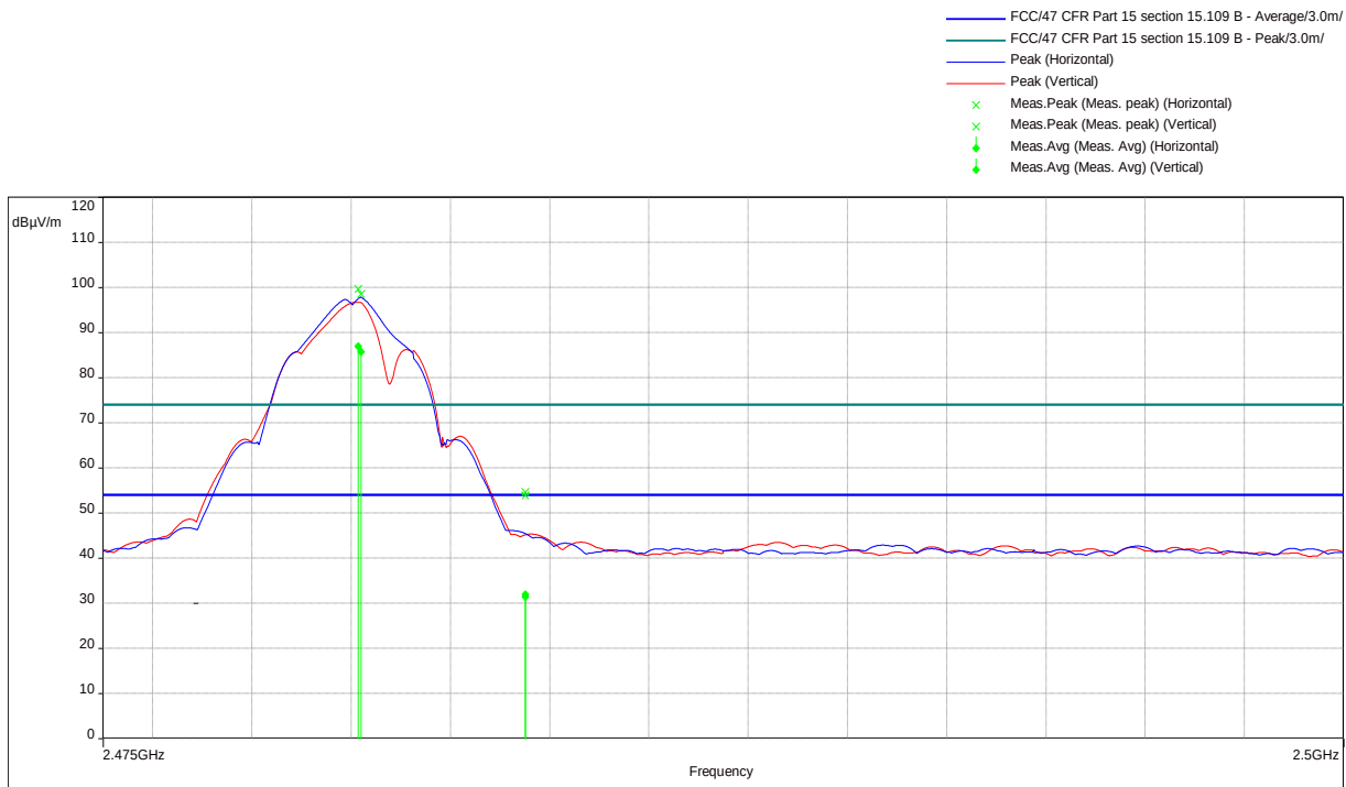
Figure 40: Band-edge-2480 MHz
