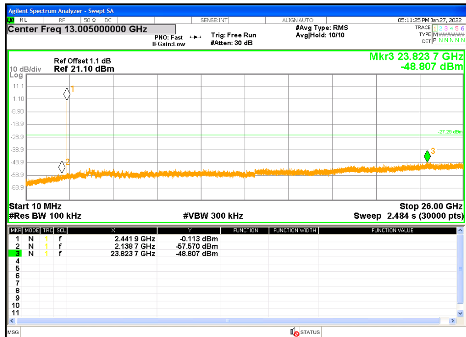
Figure 36: Out of band Emissions at 2 Mbps, 2442 MHz- Transmitter
