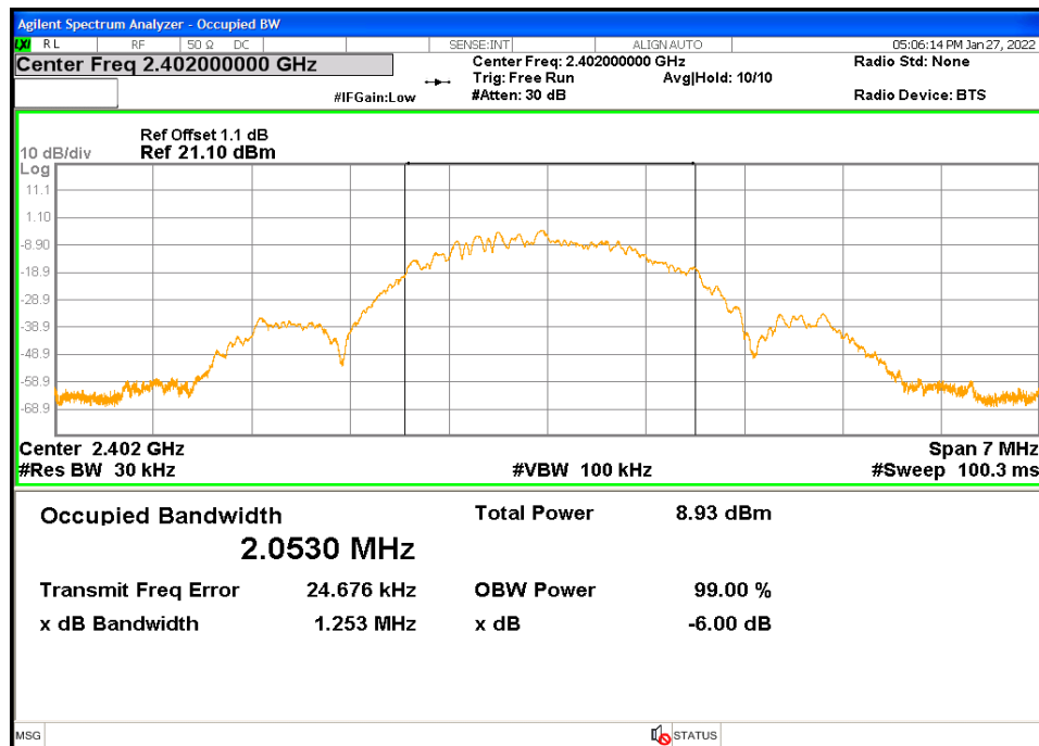
Figure 18: 99% Bandwidth - Transmitter at 2 Mbps - 2402 MHz
