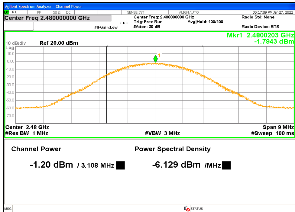
Figure 8: Maximum Transmitted Power at 2 Mbps, 2480 MHz- Transmitter
